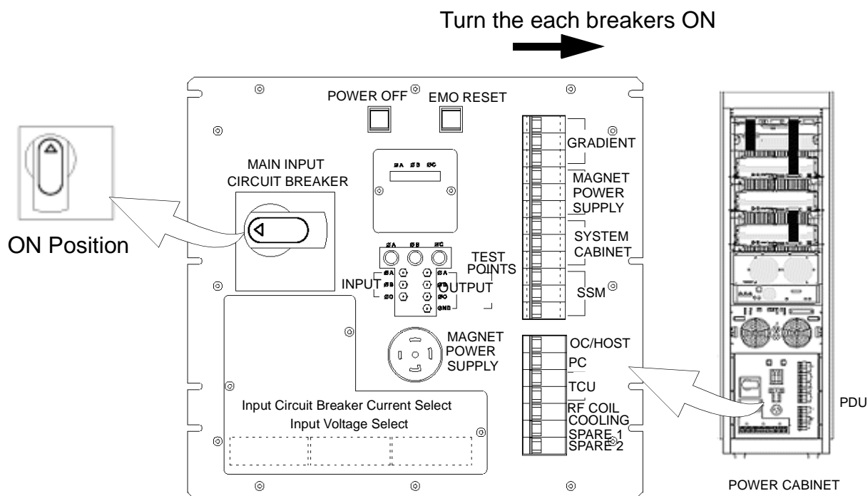
PDU FRONT PANEL ILLUSTRATION 1-1
