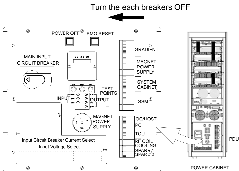
PDU FRONT PANEL ILLUSTRATION 2-1
