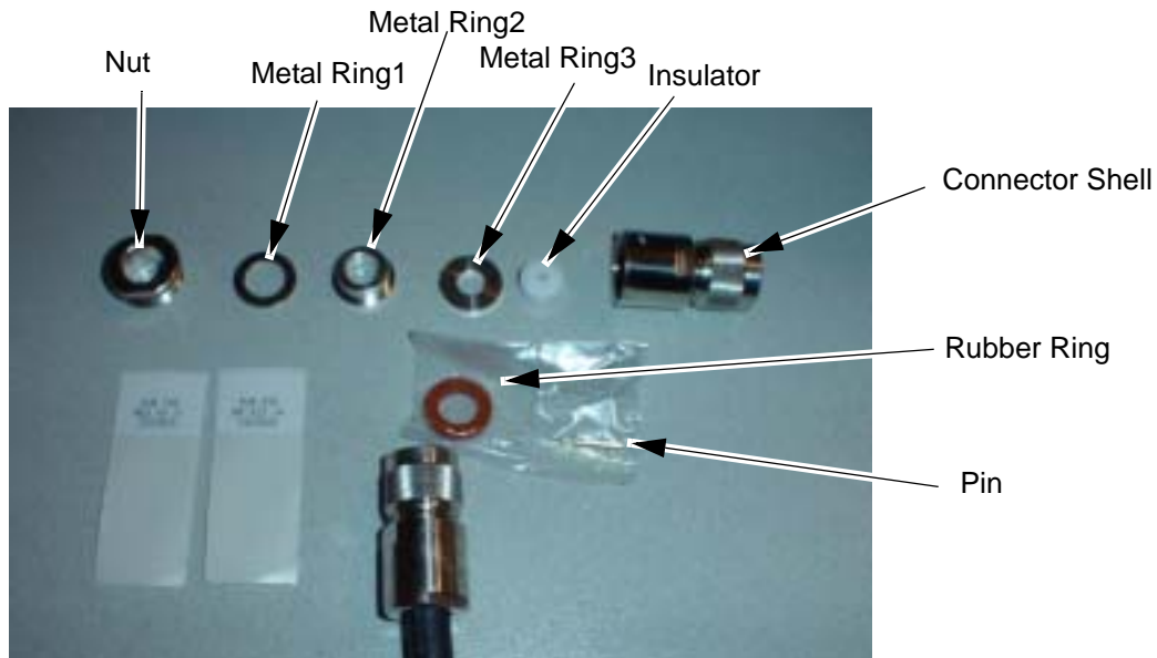
RF CABLE CONNECTOR KIT
