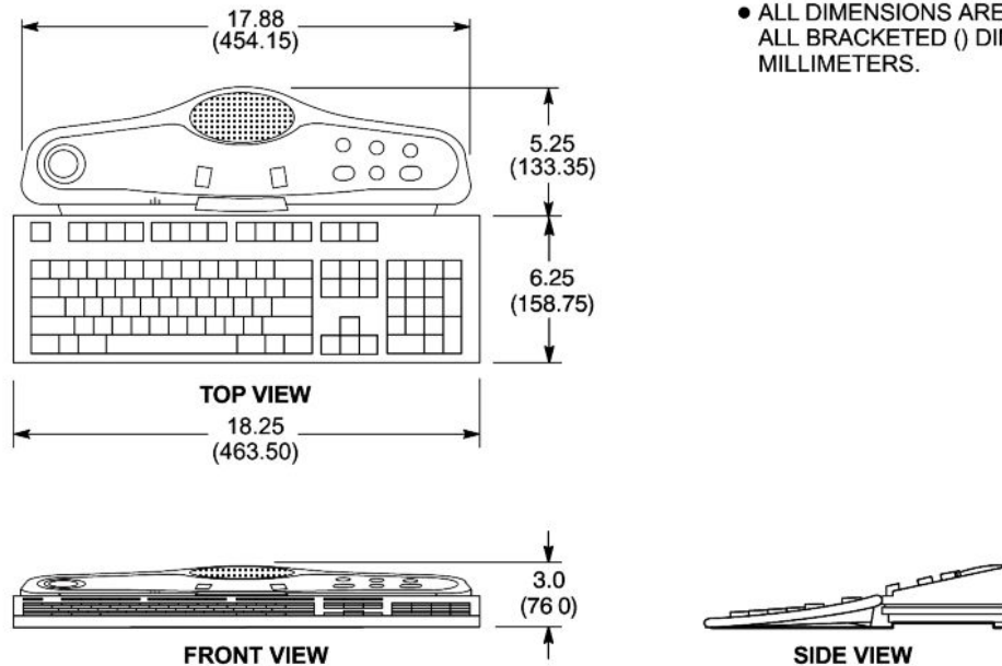
Illustration 2-32: Operator Workspace Components Position on Table Top - Keyboard
