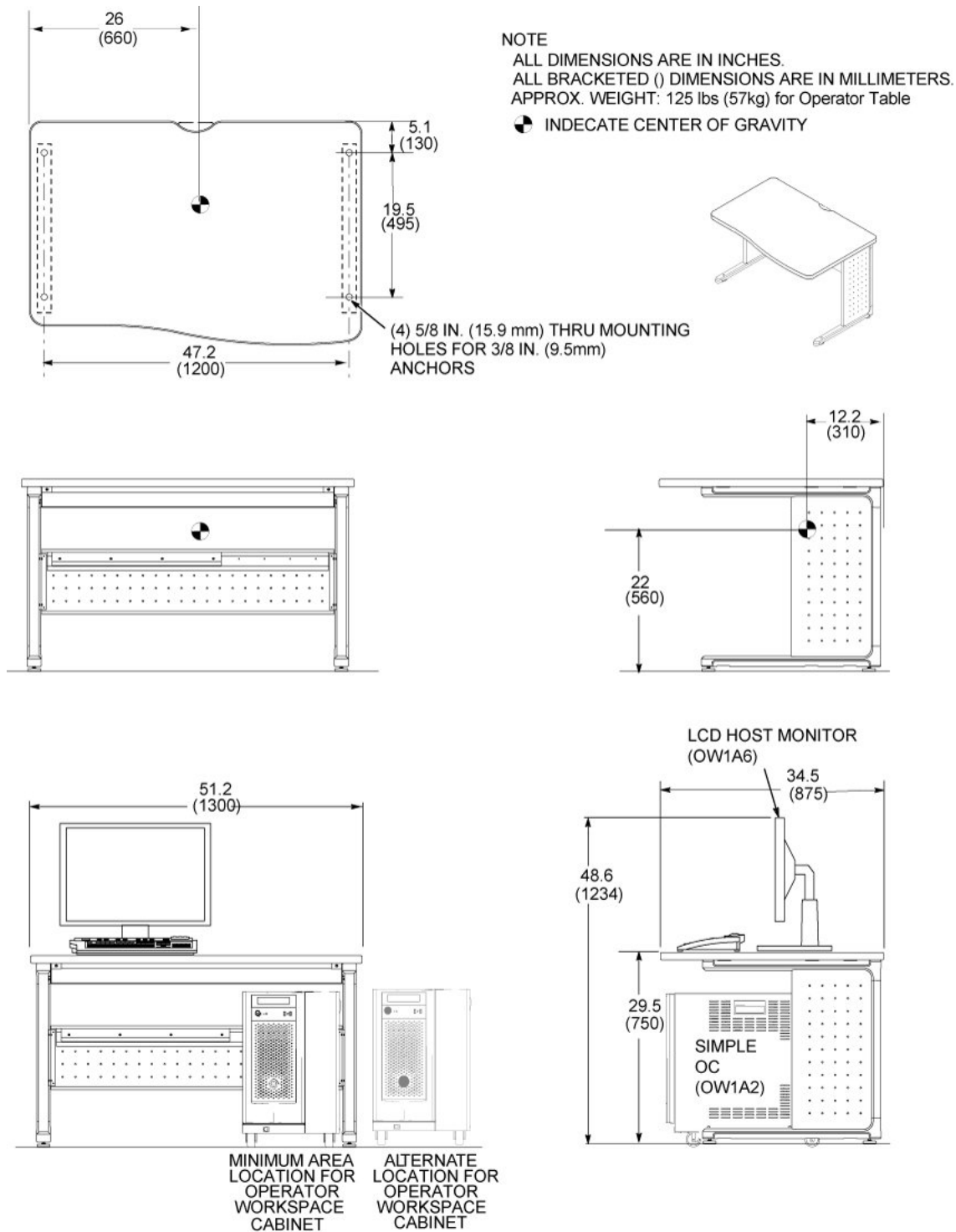
Illustration 2-29: Operator Workspace (OW1) Overall Dimensions
