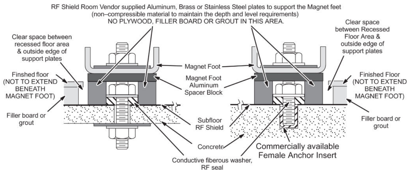
Illustration 2-47: Magnet Anchor Details
