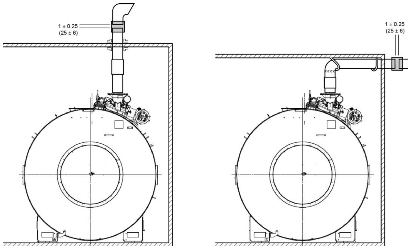
Illustration 4-19: Outside Dielectric Break (Customer-supplied)
