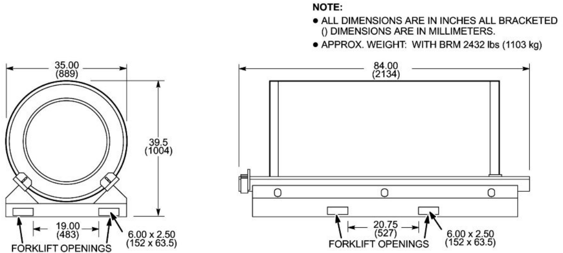
Illustration 1-4: Short Room Replacement BRM Gradient Coil Assembly & Cradle On Cart
