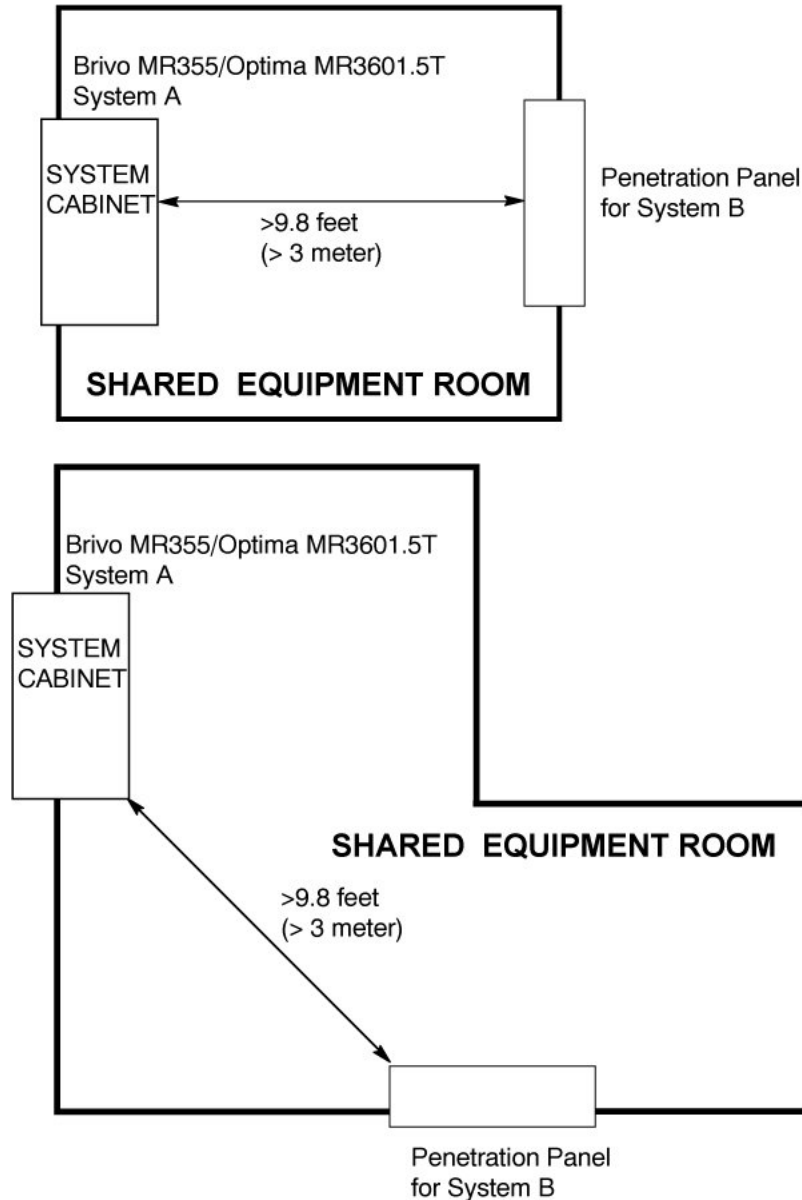
Illustration 2-44: Multiple MR Systems Penetration Panel Spacing
