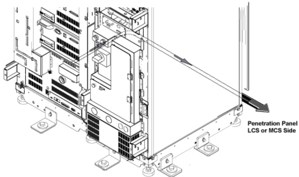
Illustration 2-53: Rear Hose Routing
