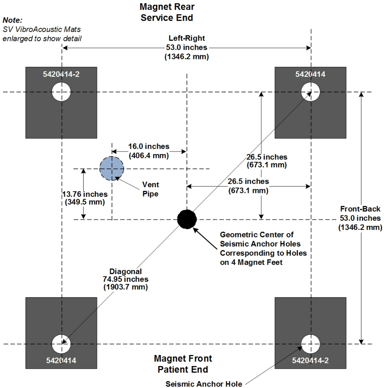
Illustration 2-60: Positioning SV VibroAcoustic Mats
