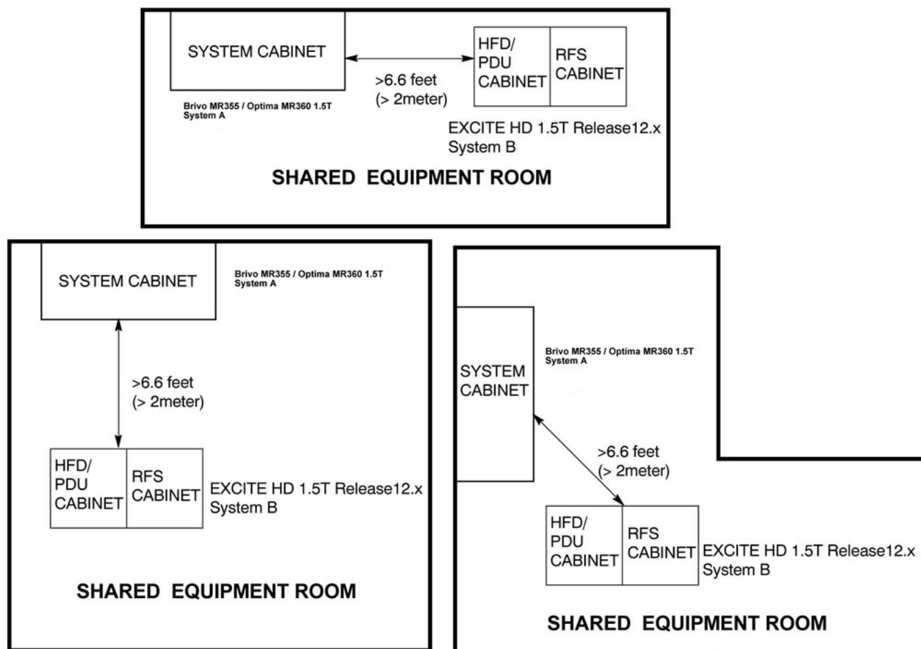
Illustration 2-43: Brivo MR355 / Optima MR360 & Excite(Release 12.x) Systems Electronics Cabinets Spacing
