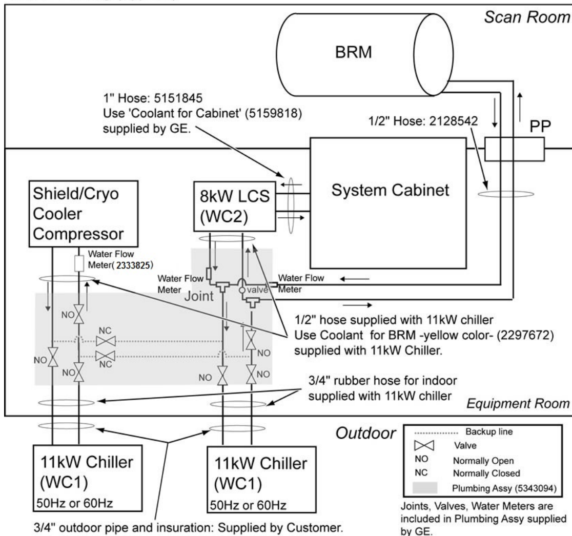
Illustration 4-2: Type A Chiller Configuration
