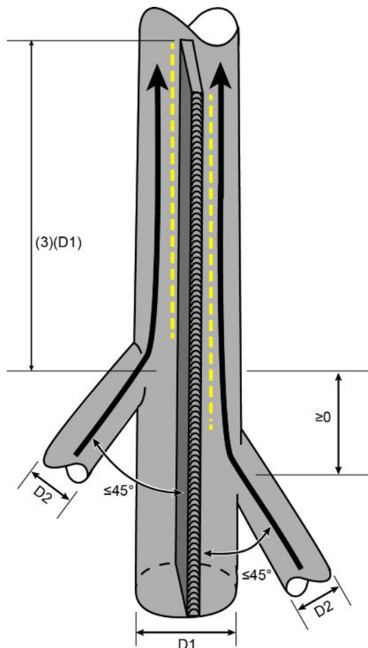
Illustration 4-22: Combined Vent
