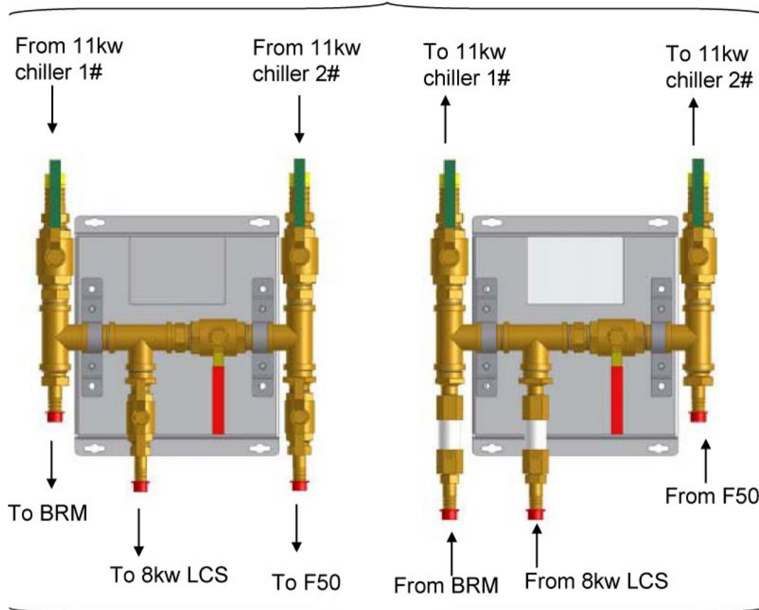
Illustration 4-3: Plumbing Assy for Type A
