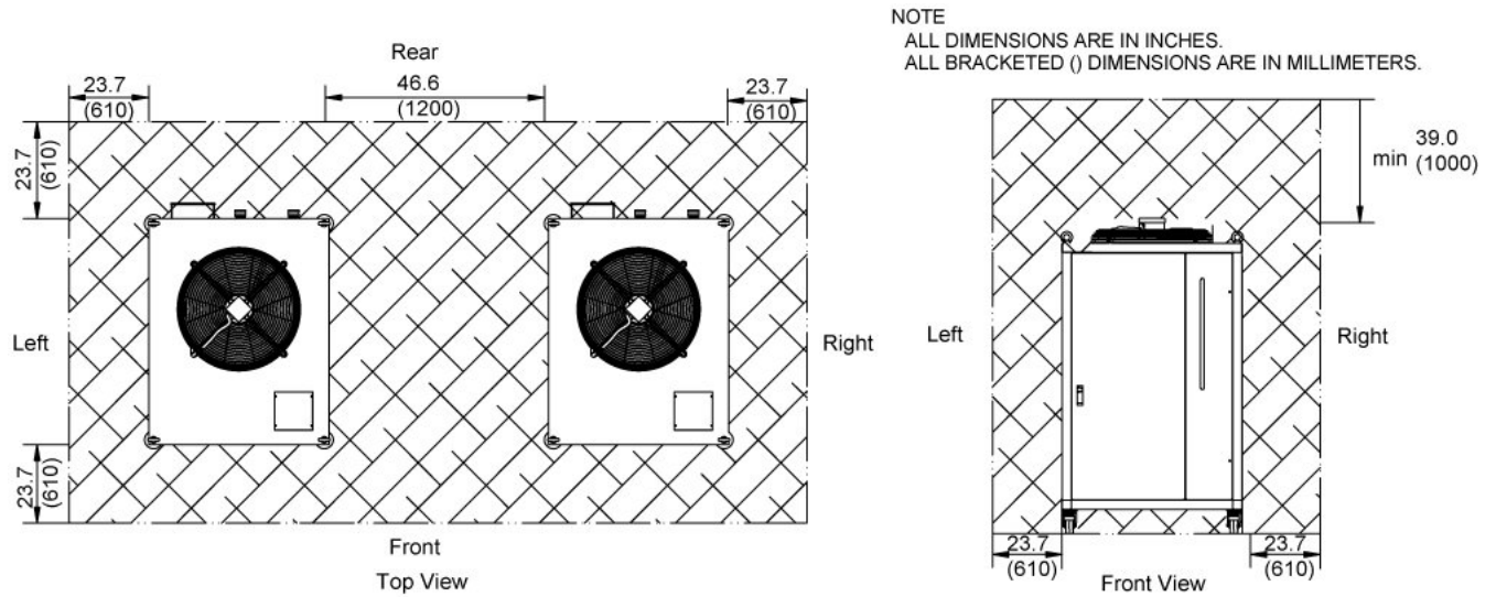
Illustration 2-38: Service Clearances for two or more units 2
