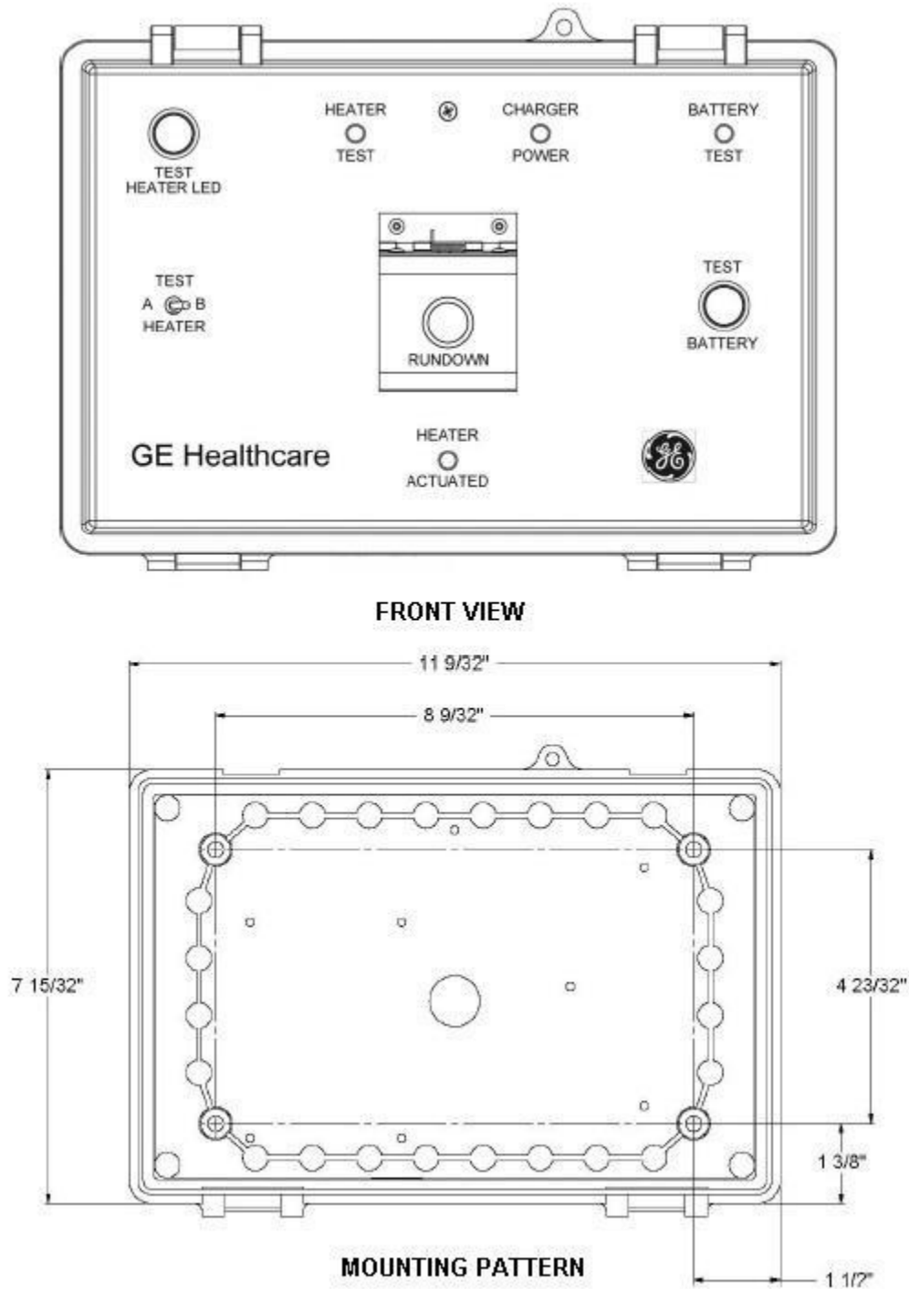
Illustration 2-13: Front View and Mounting Pattern
