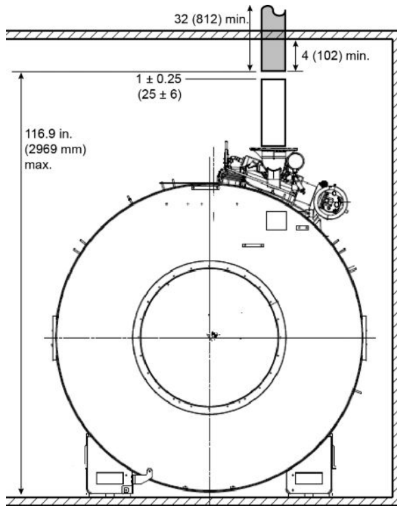
Illustration 4-18: Pipe Supports to Remove Vent Load from Ventglas Connection
