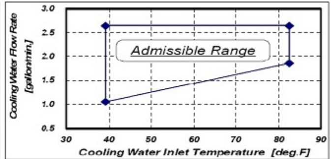
Illustration 4-13: Cooling Water Typical Flow Characteristics
