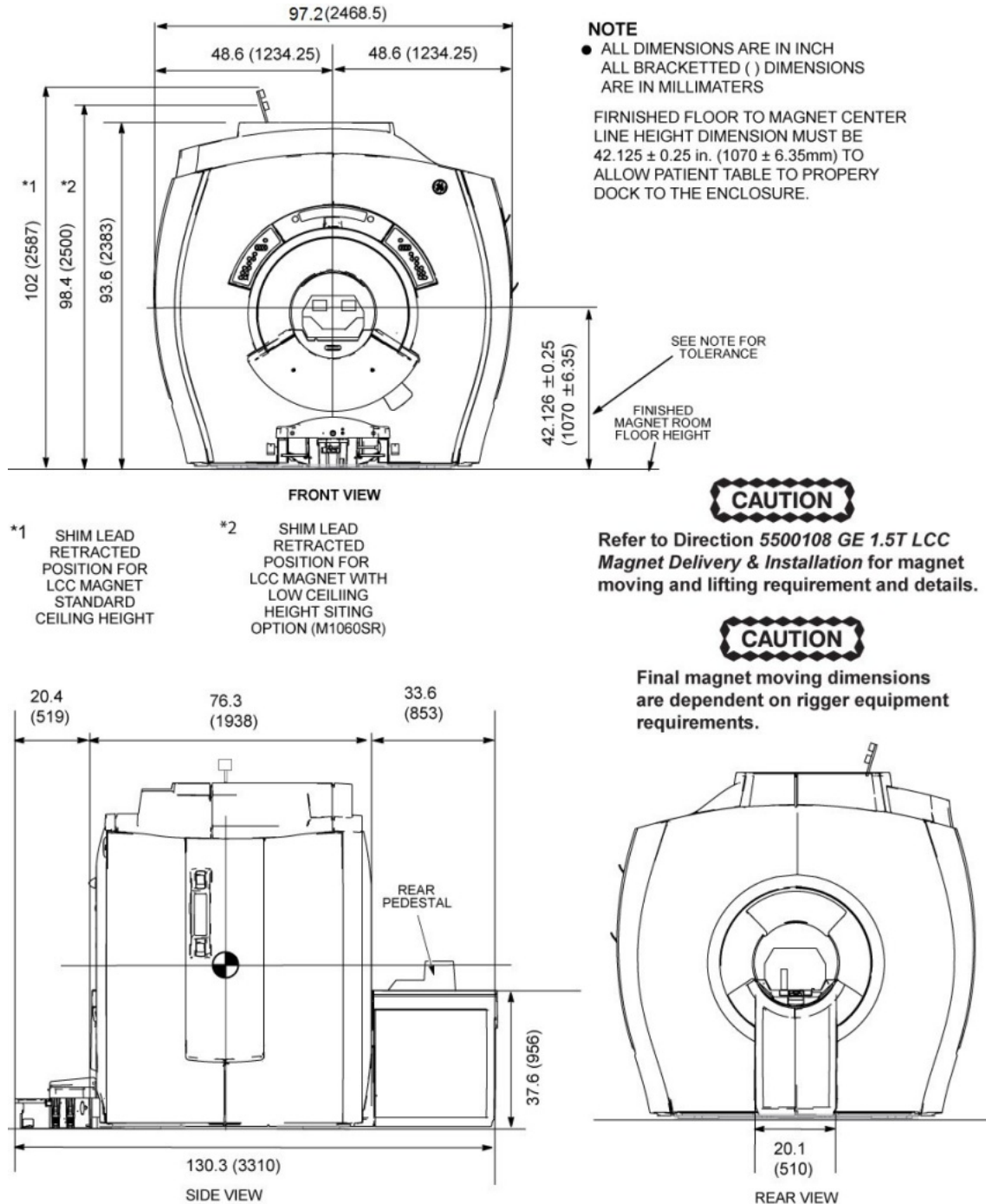
Illustration 2-6: Magnet Enclosure Dimensions
