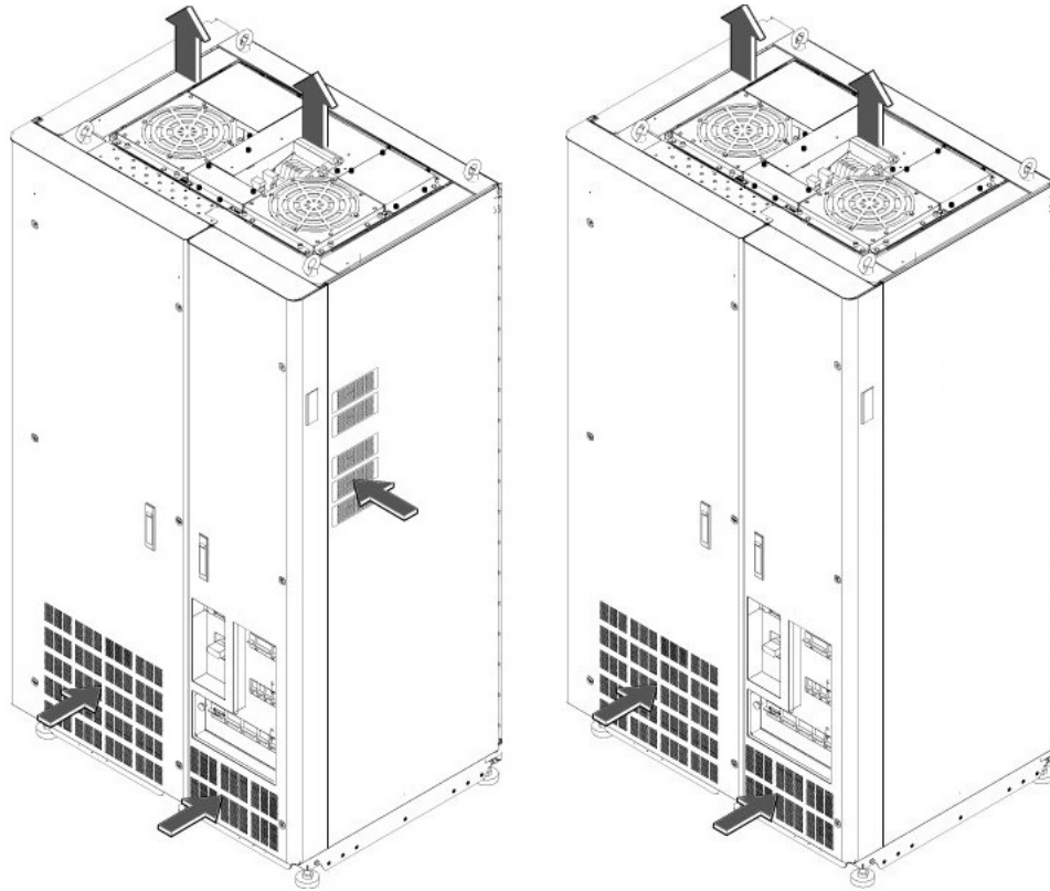
Illustration 2-56: System Cabinet Air Flow
