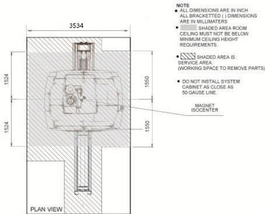
Illustration 2-48: Minimum Ceiling Height for Magnet Servicing
