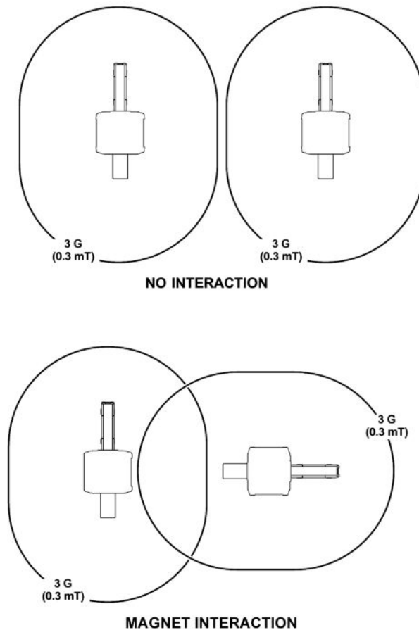
Illustration 2-42: Two Magnet Installation
