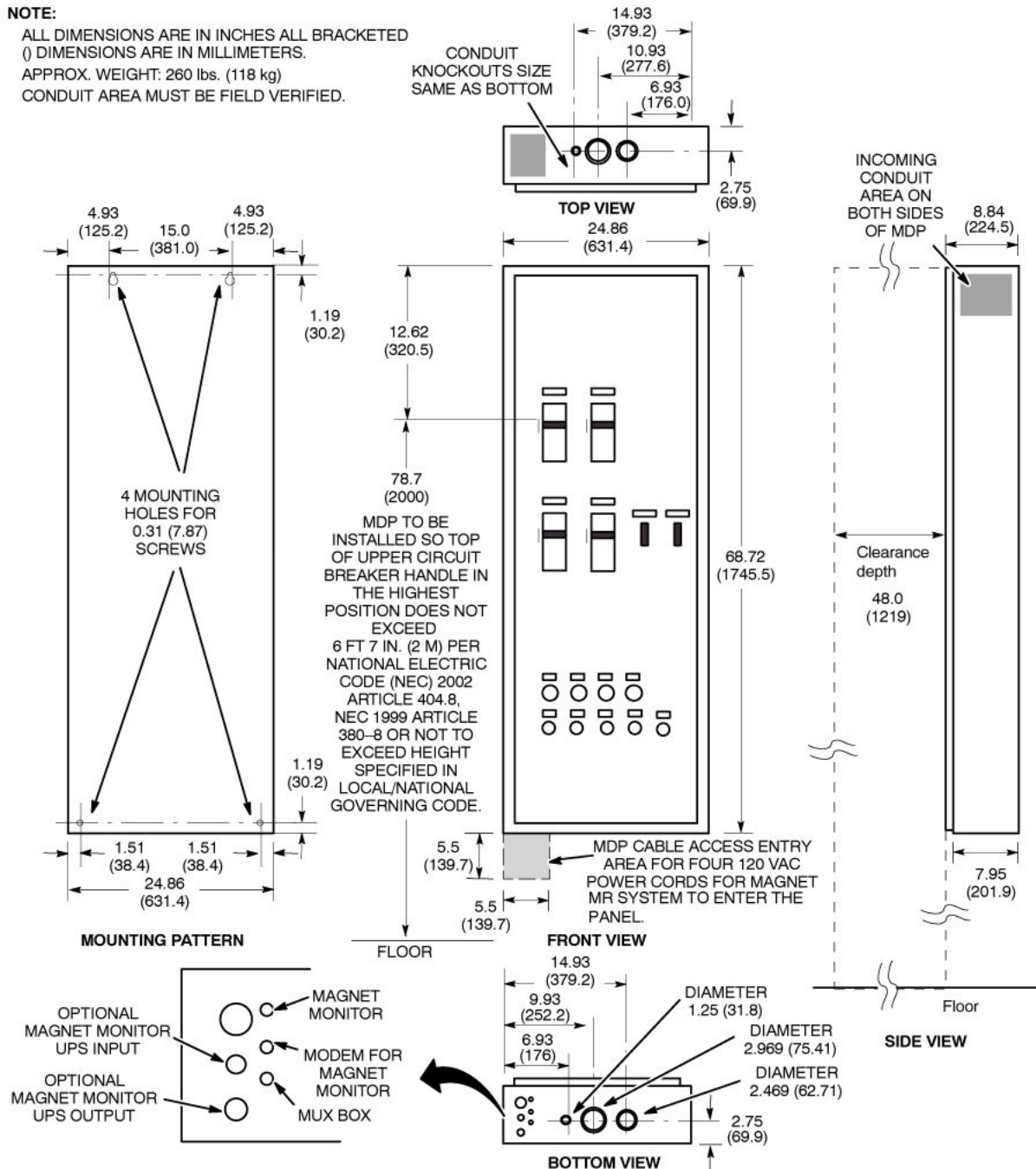
Illustration 2-21: Main Disconnect Panel (MDP) M3088TM Option
