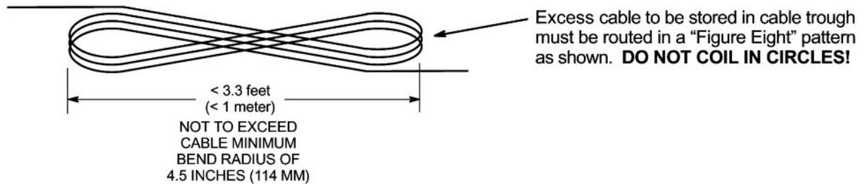
Illustration 2-45: Proper Storage Of Excess Receive Cables
