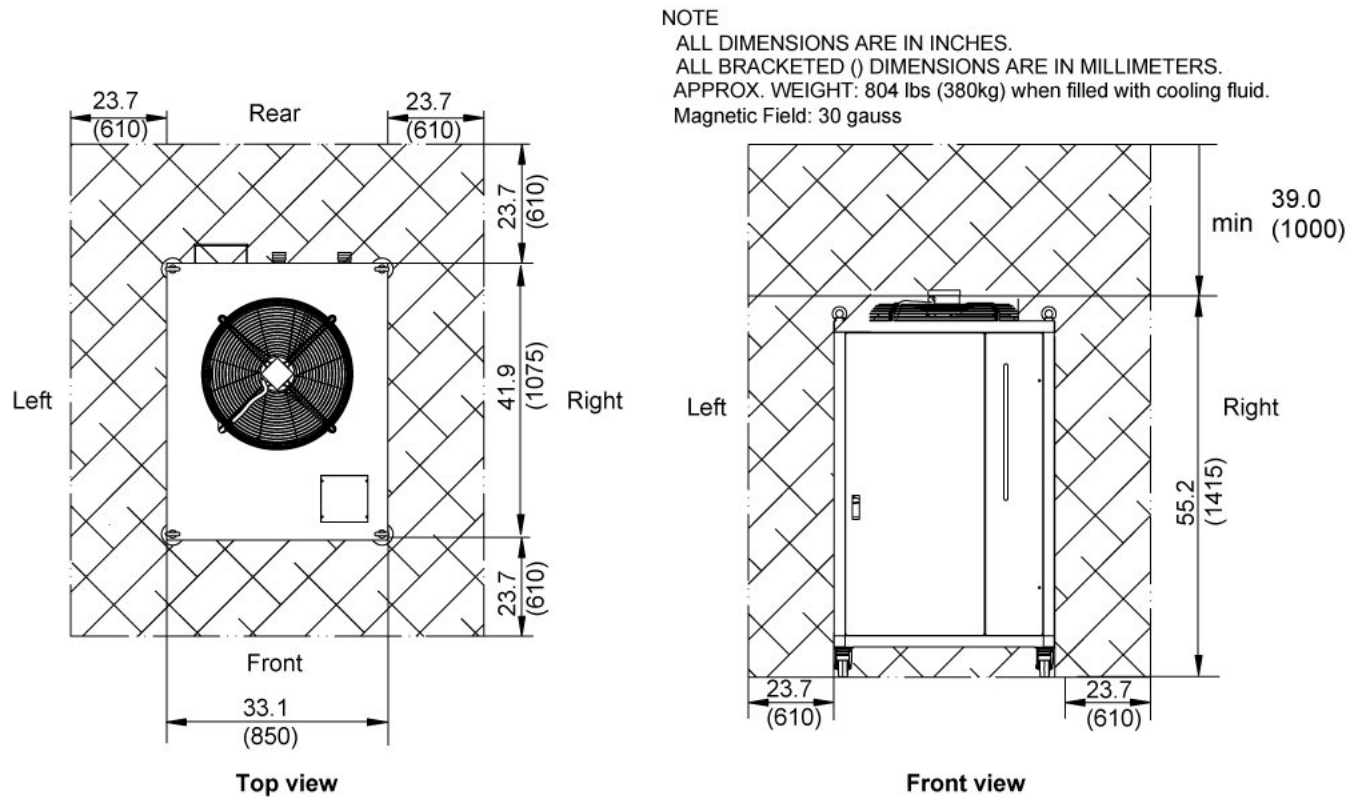
Illustration 2-36: 11kW Airsys Water Chiller Dimensions and Service Clearance for single unit
