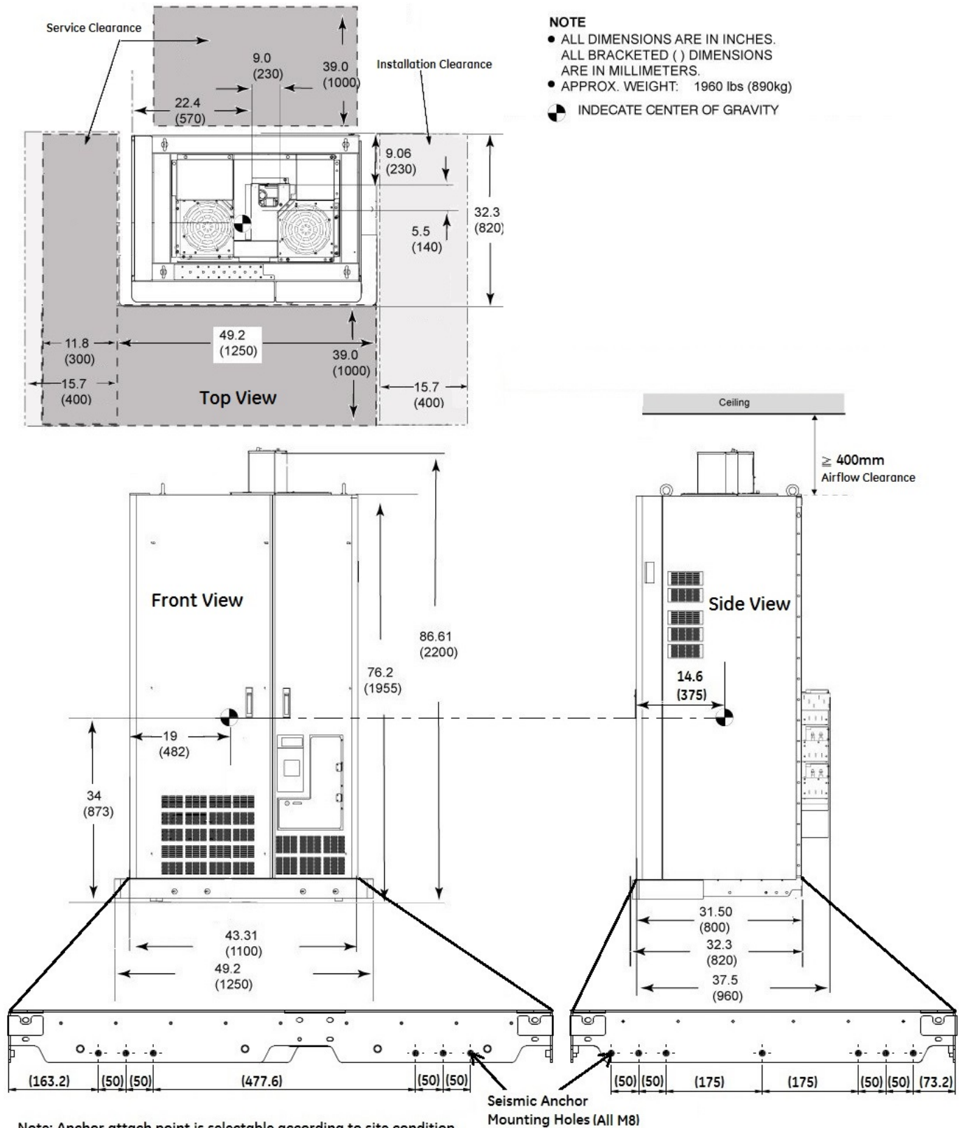
Illustration 2-17: System Cabinet
