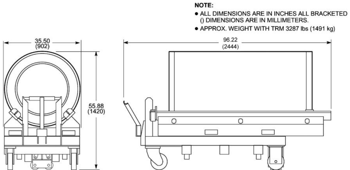
Illustration 1-4: Short Room Replacement BRM Gradient Coil Assembly & Cradle On Cart
