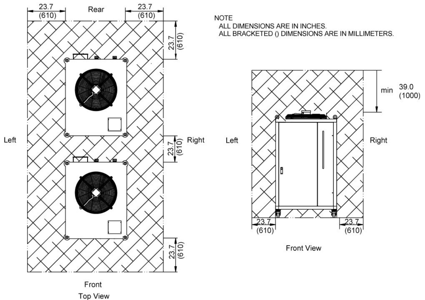
Illustration 2-38: Service Clearances for two or more units 2
