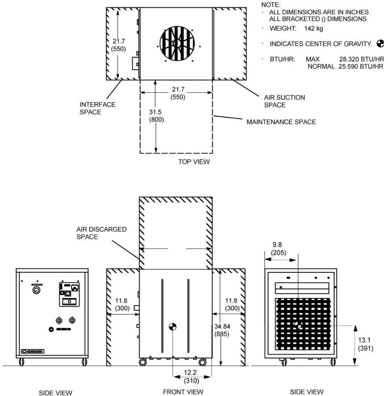
Illustration 2-23: CSA-71A COMPRESSOR UNIT for 200V Site Only
