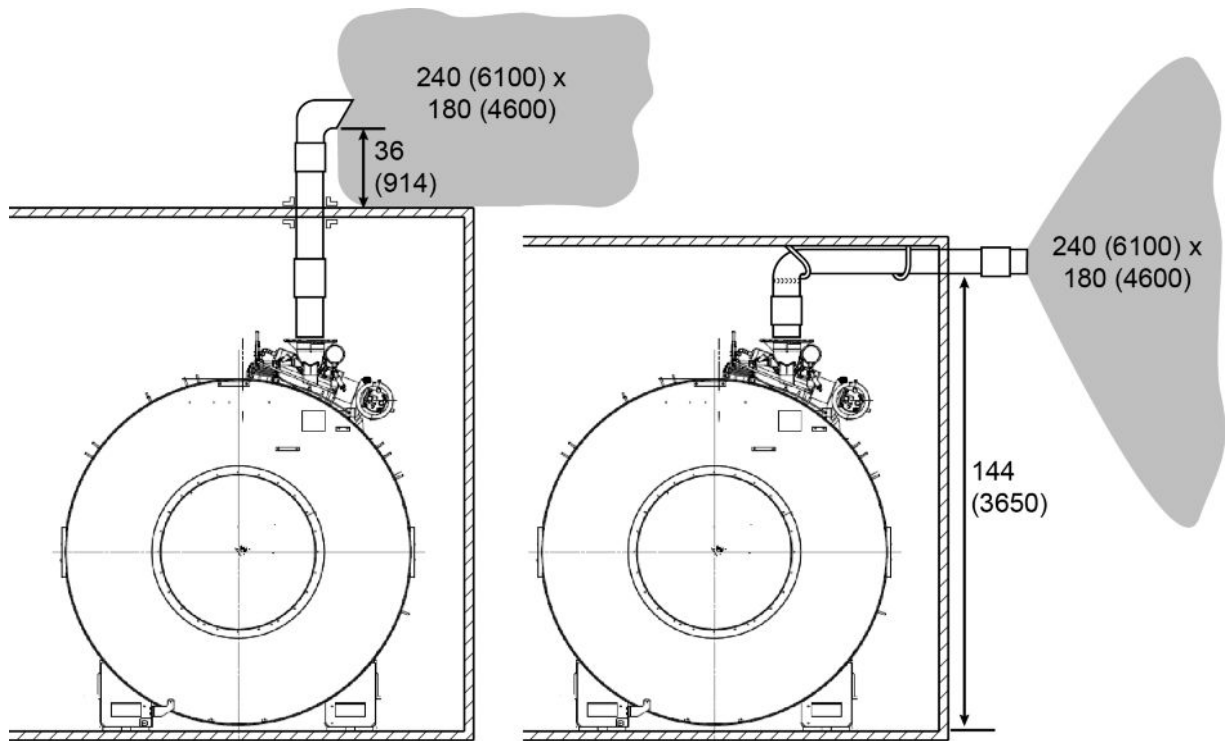
Illustration 4-20: Cryogenic Exterior Venting Volume
