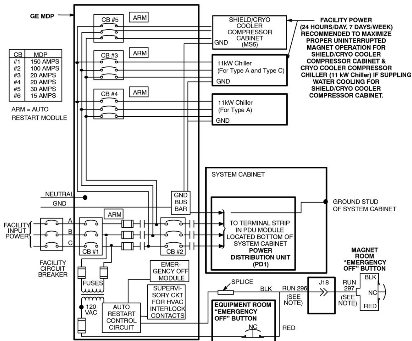
Illustration 5-1: GE pre-engineered MDP (M3088TM) schematic for Type A, B or C configuration
