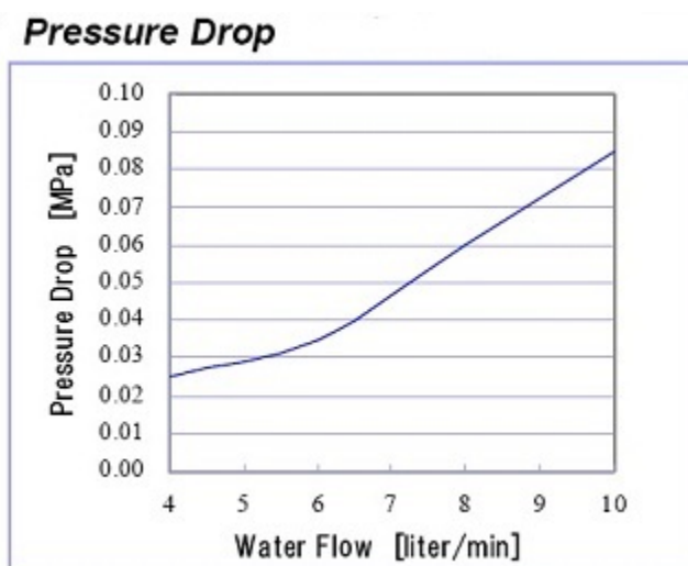
Illustration 4-12: Cooling Water Typical Flow Characteristics
