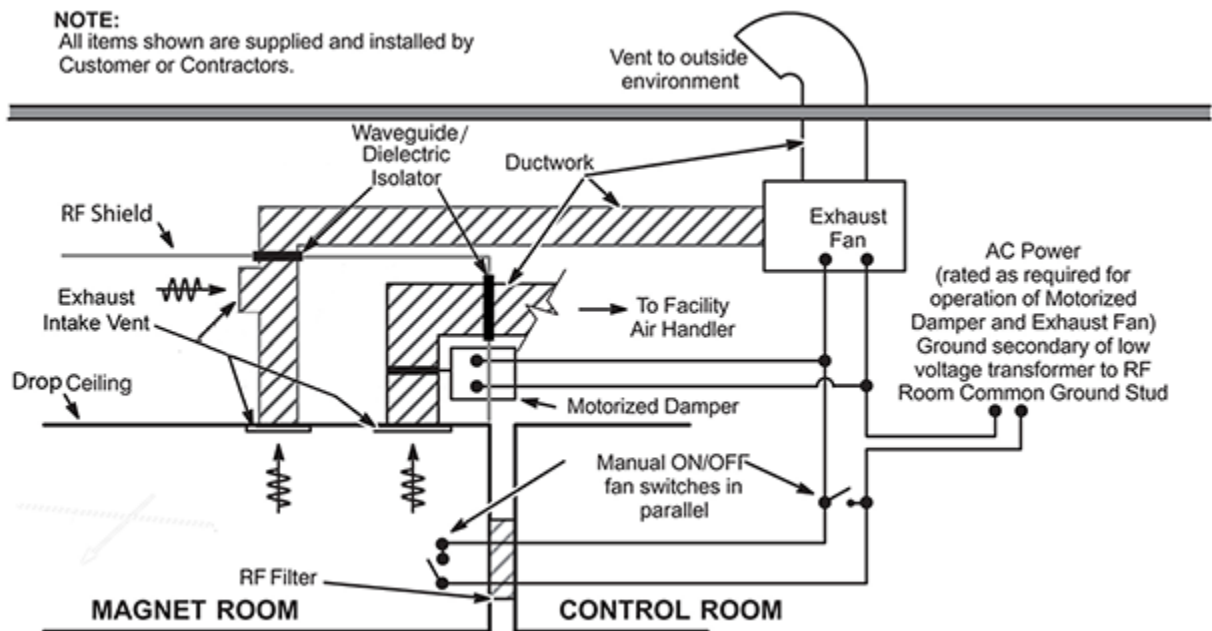
Illustration 4-14: Magnet Room Exhaust Fan Schematic
