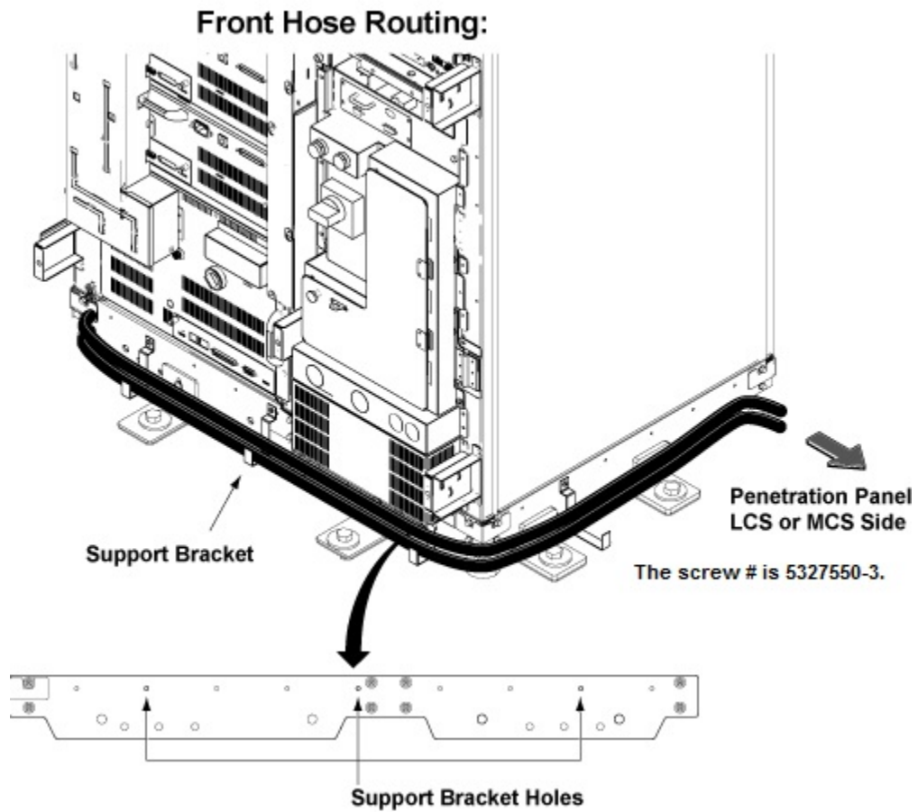
Illustration 2-54: Front Hose Routing
