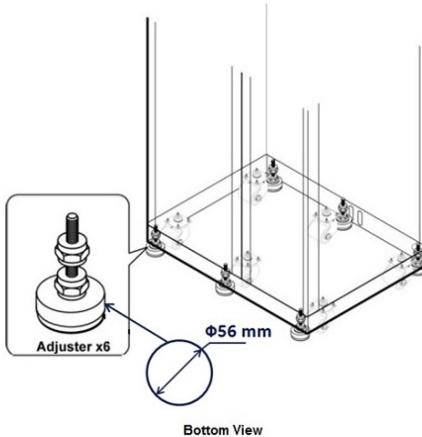
Illustration 2-16: System Cabinet Floor Support
