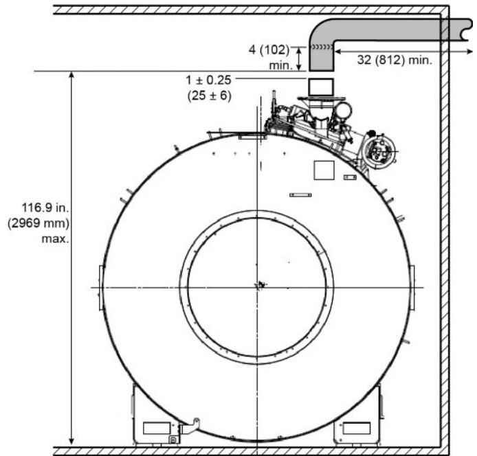
Illustration 4-18: Pipe Supports to Remove Vent Load from Ventglas Connection
