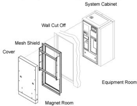
Illustration 2-19: Mesh Shield and System Cabinet Cover
