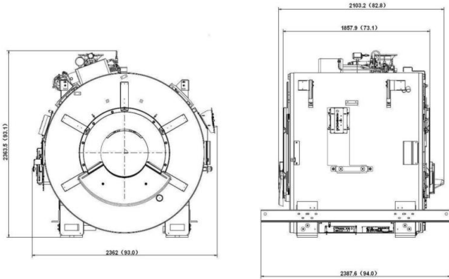
Illustration 1-2: Magnet Size for Transportation
