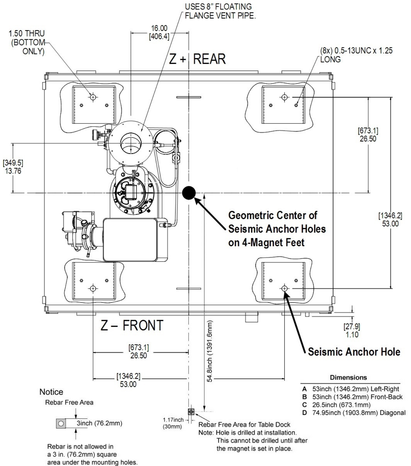
Illustration 2-59: 1.5T LCC Magnet Geometry, R Series
