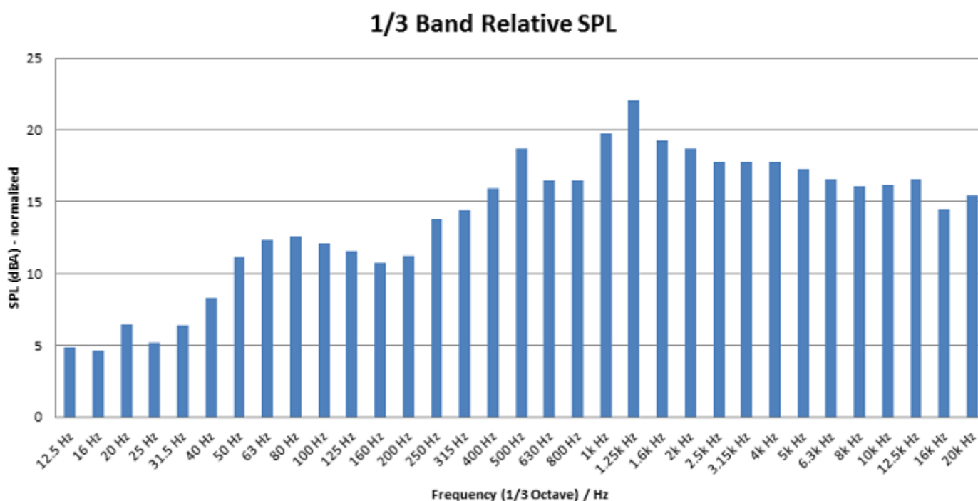
Illustration 2-57: Sound Pressure Spectral Distribution (1/3 Band Relative SPL)
