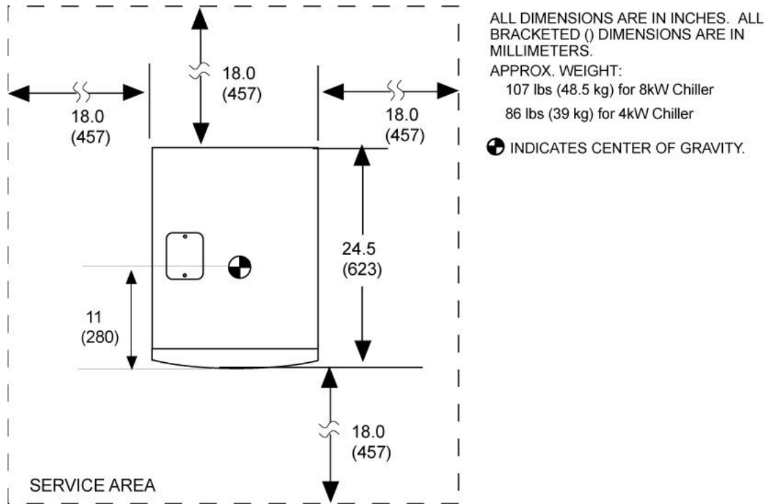
Illustration 2-26: Water Chiller For System Cabinet
