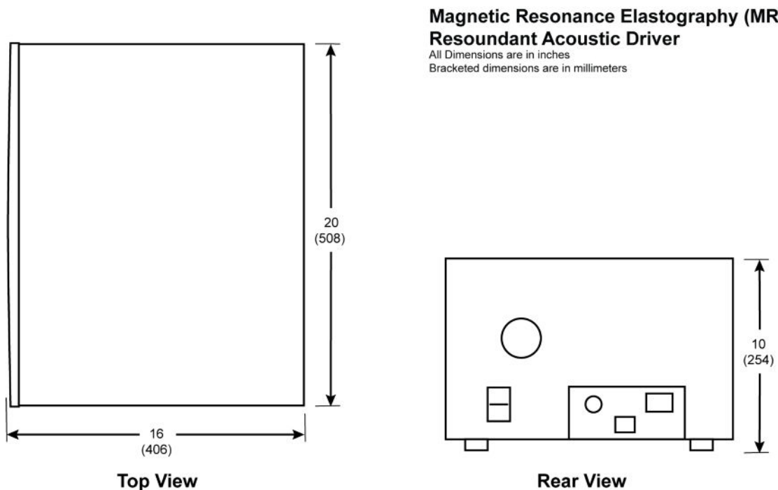
Illustration 2-41: Magnetic Resonance Elastography (MRE) Resoundant Acoustic Driver
