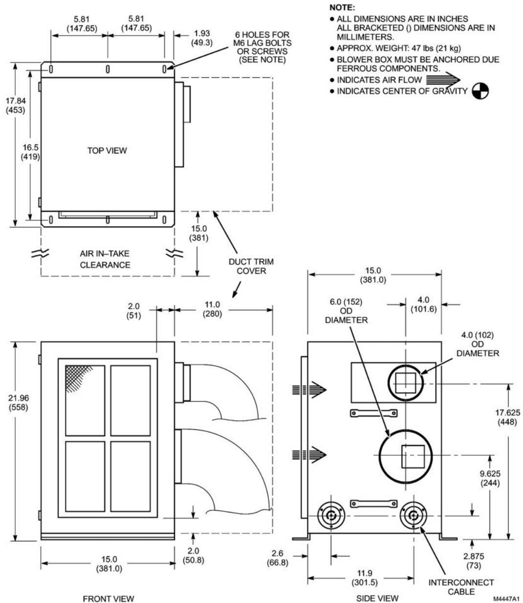
Illustration 2-15: Blower Box (MG6)
