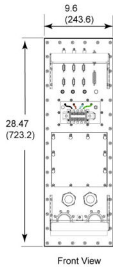
Penetration Panel
