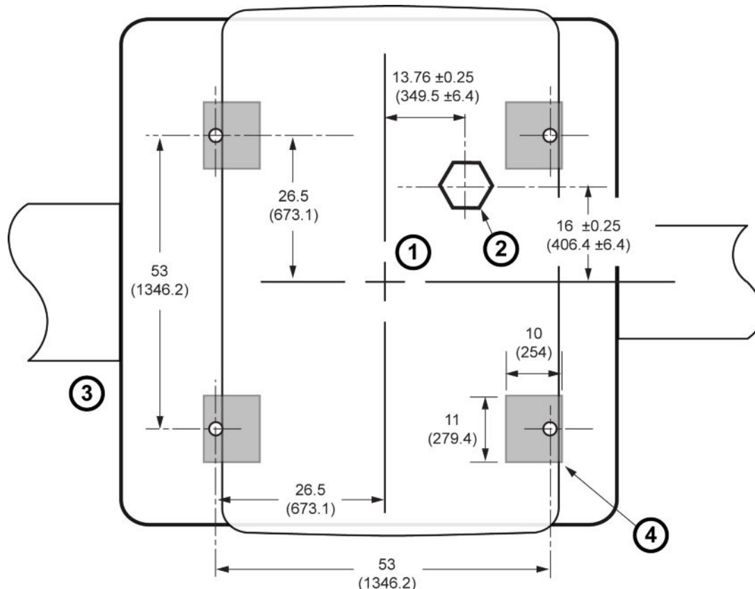
Illustration 4-21: Magnet Cryogenic Vent Location
