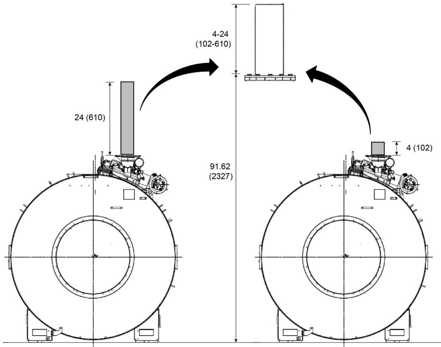
Illustration 4-16: Flanged Magnet Vent Adapter
