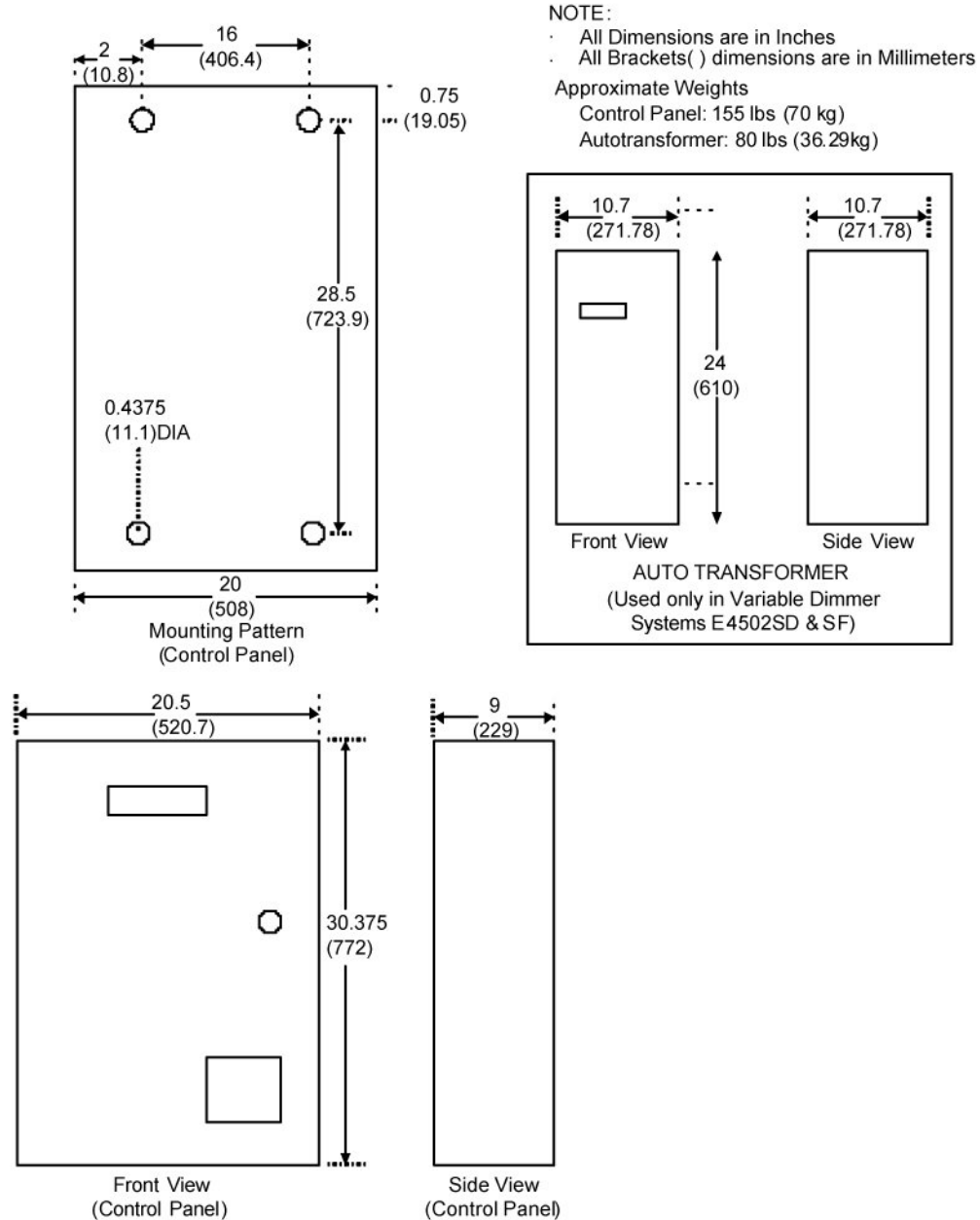
Illustration 2-25: DC Lighting Controller Option
