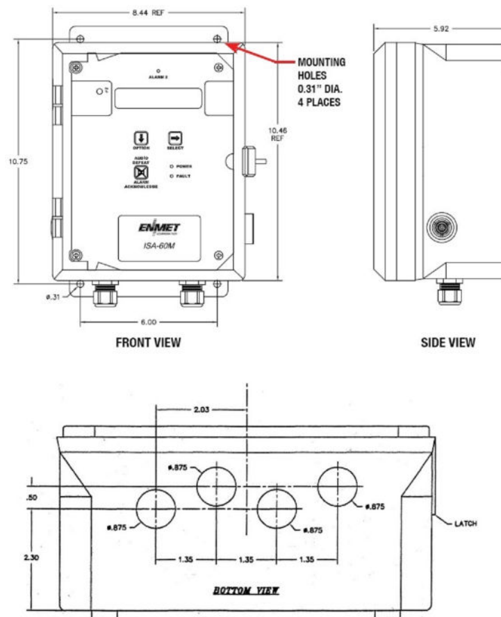
Illustration 2-34: Oxygen Monitor (OM1)
