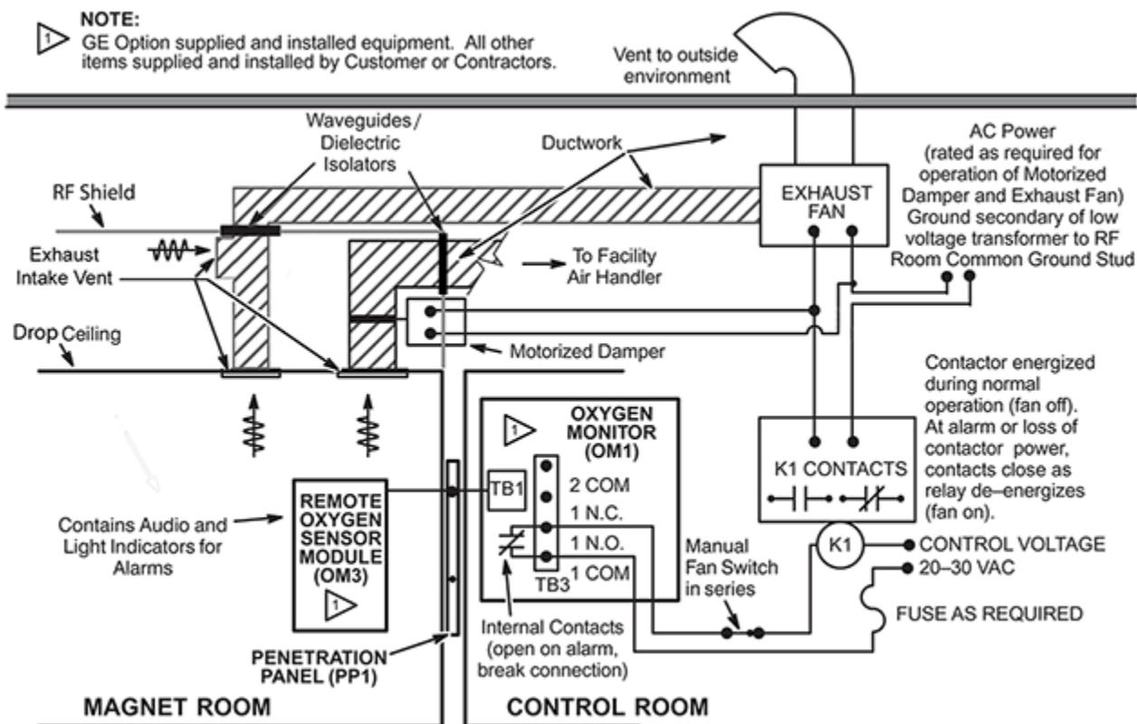
Illustration 4-15: Magnet Room Exhaust Fan Schematic with Optional Oxygen Monitor
