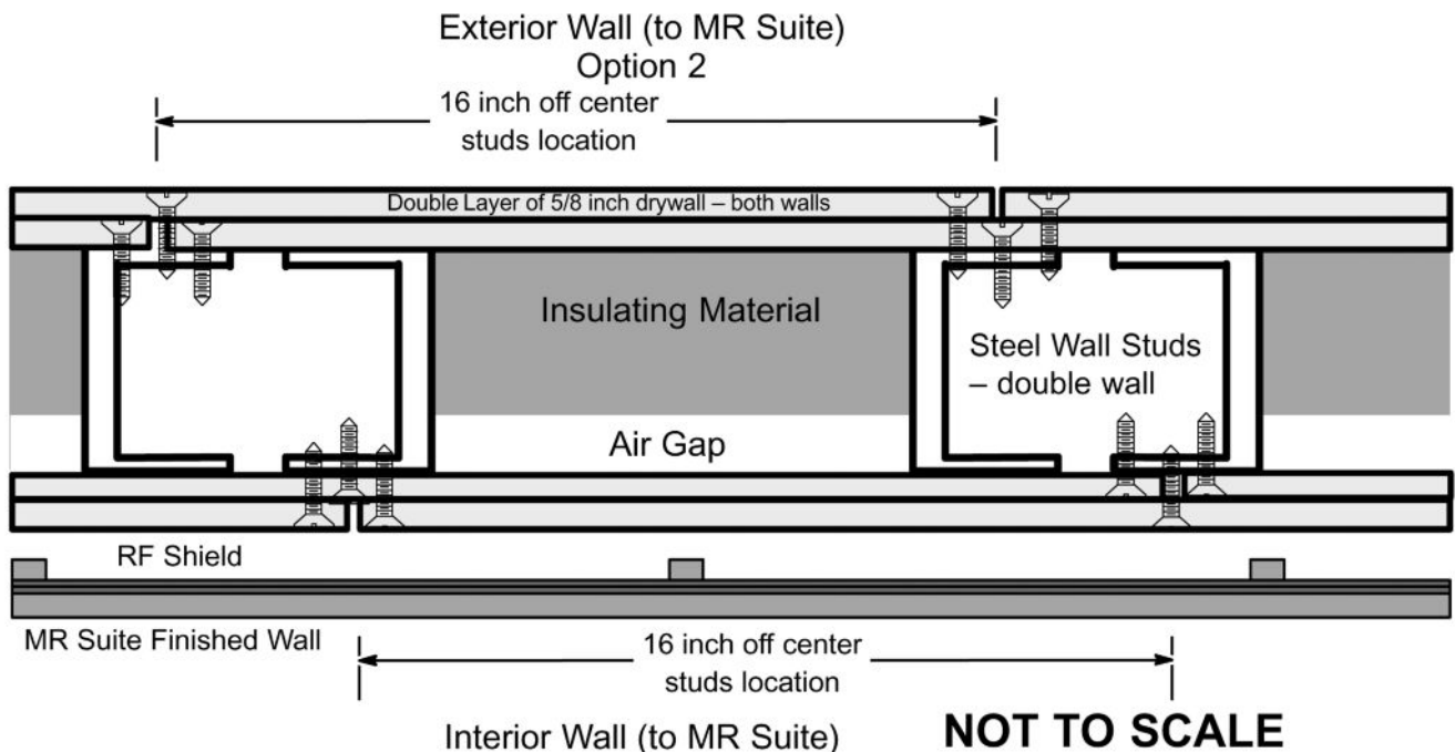
Illustration 7-7: Example Of Wall Construction For Airborne Noise Control - Option 2
