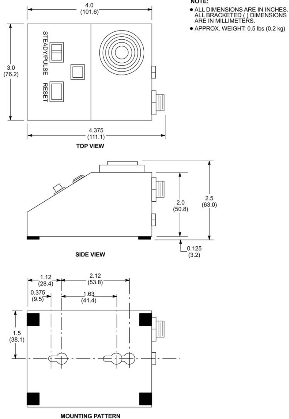
Illustration 2-33: Pneumatic Patient Alert Control Box (PA1)
