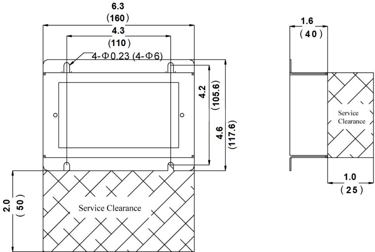
Illustration 2-40: Remote Control Panel (RCP) For 11kW Chiller
