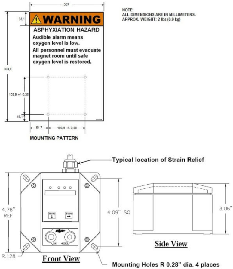
Illustration 2-35: Remote Oxygen Sensor Module (OM3)
