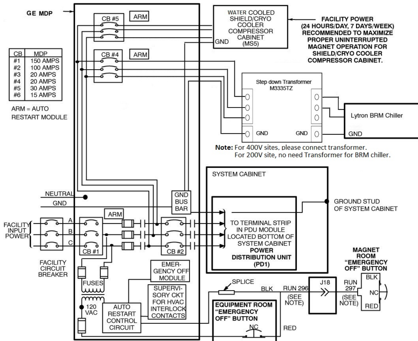
Illustration 5-3: Step down transformer connected method with customer provided MDP (Type E)
