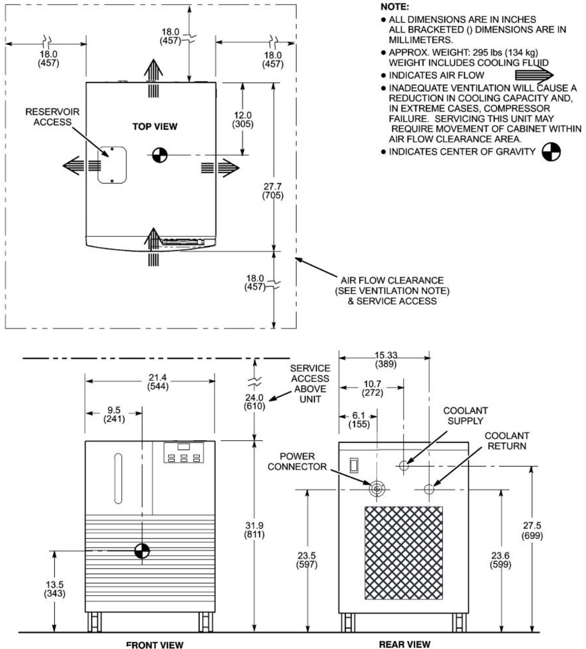
Illustration 2-28: Water Chiller (WC1) For BRM Gradient Coil Cooling Water
