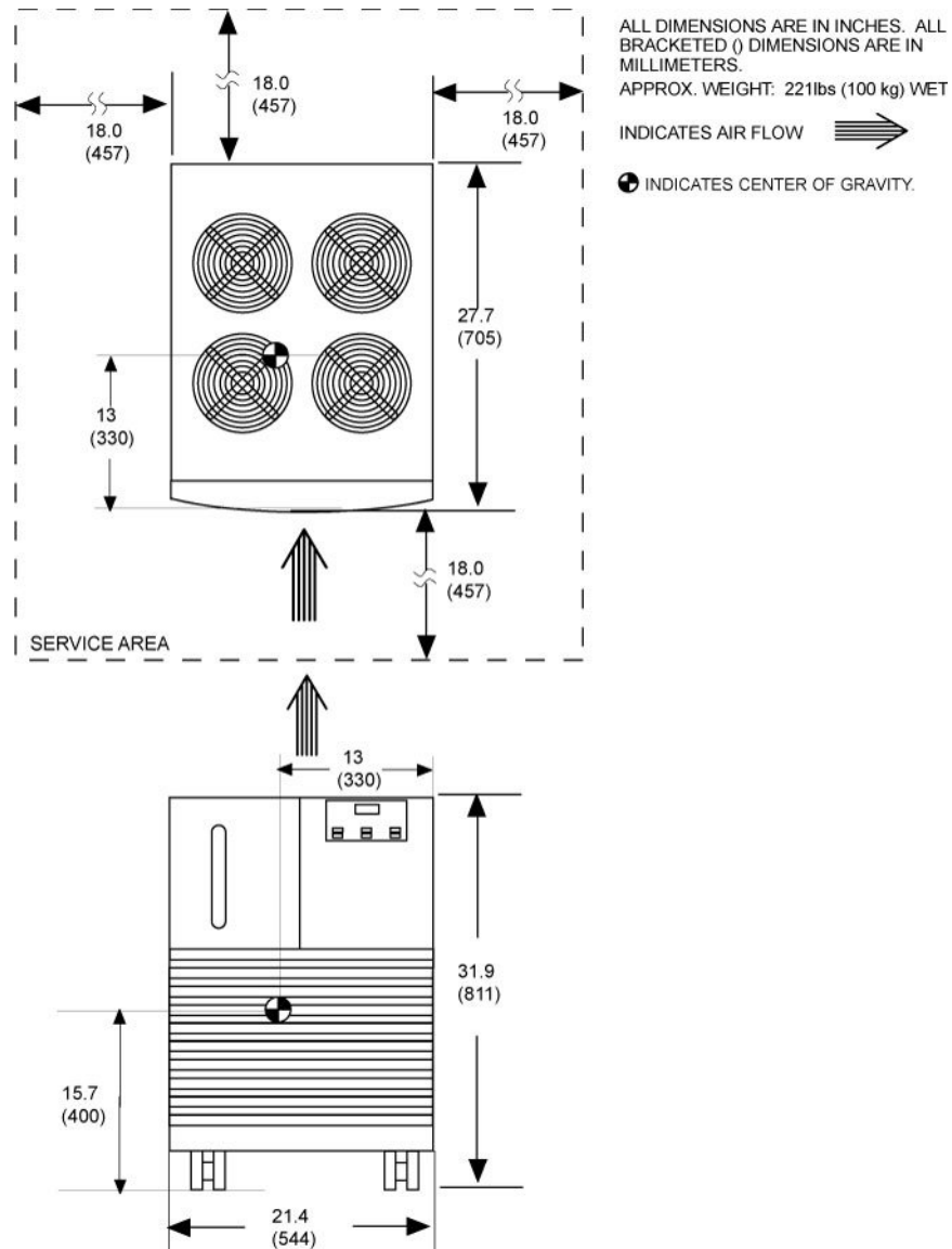
Illustration 2-27: Water Chiller (WC2) For System Cabinet
