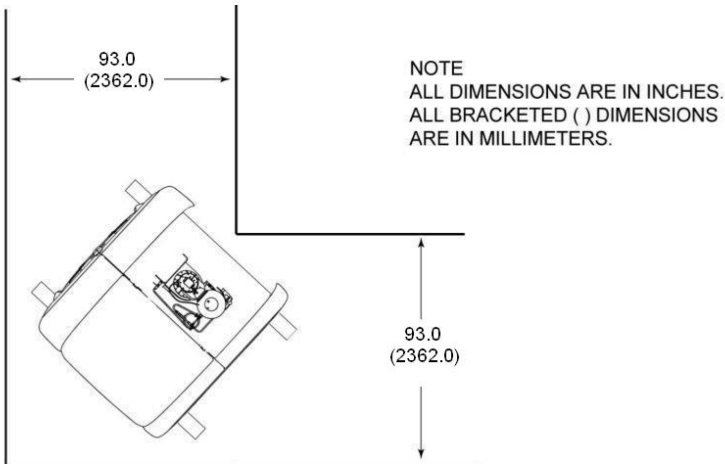
Illustration 1-1: LCC Magnet Minimum Door/Hallway Dimensions 90° Turn
