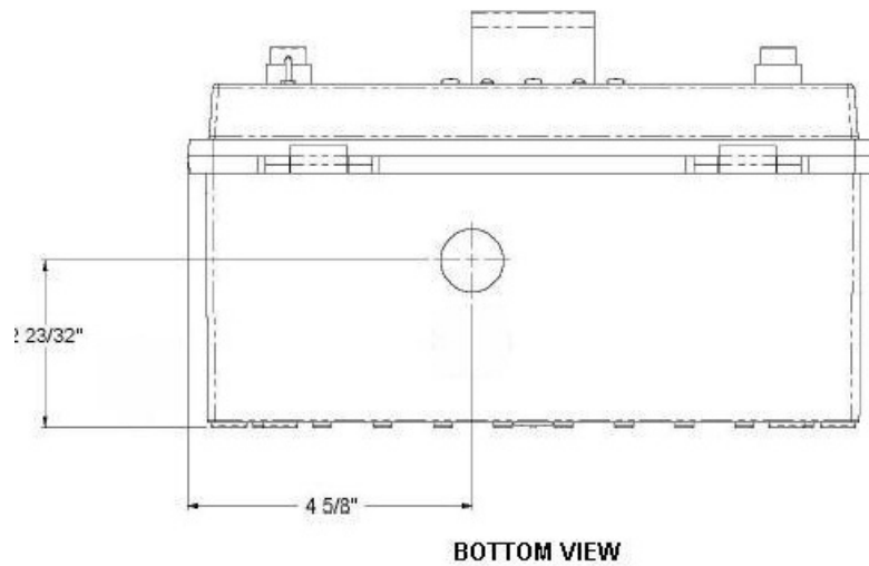
Illustration 2-14: Bottom View
