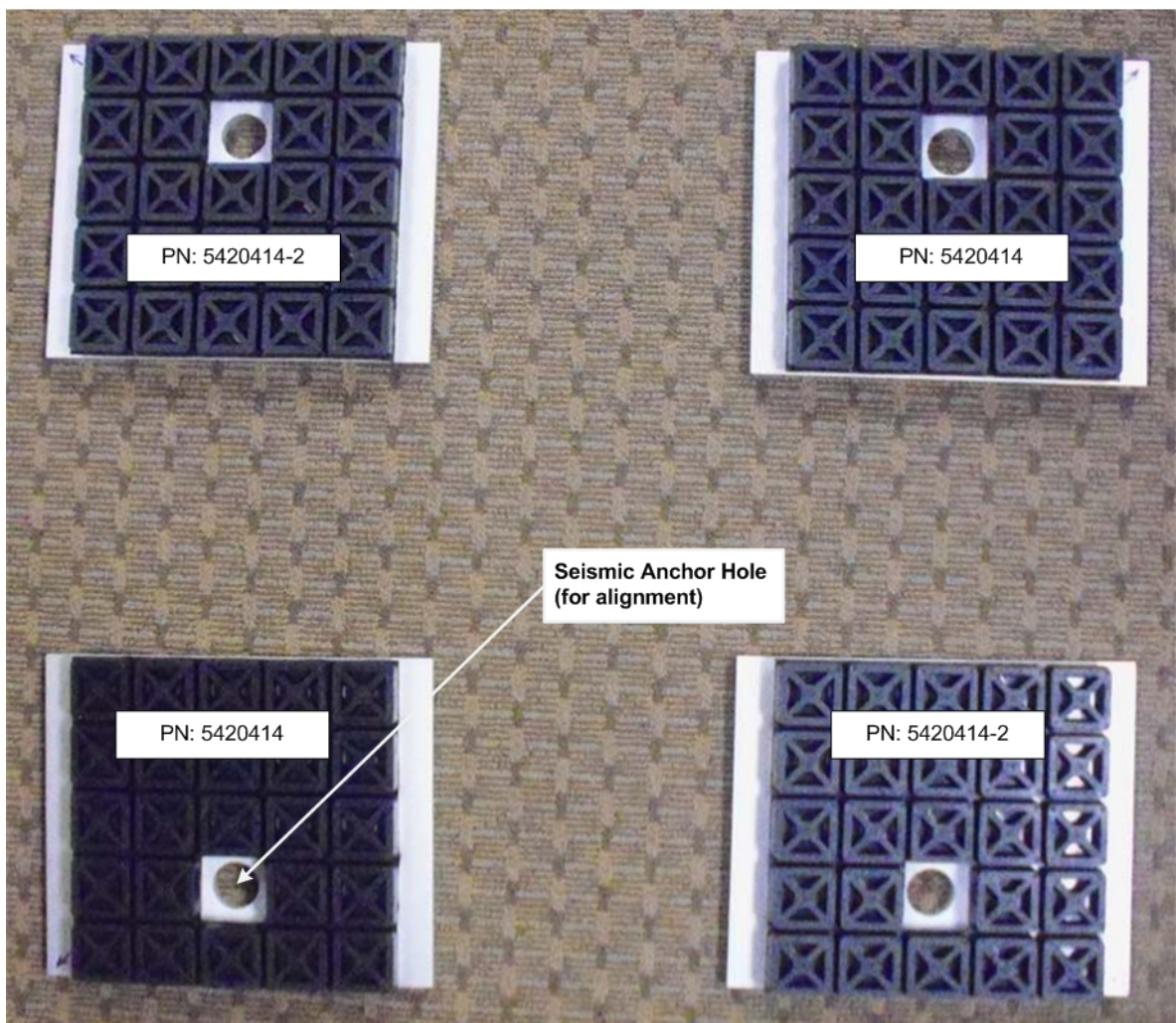
Illustration 2-62: SV VibroAcoustic Mats
