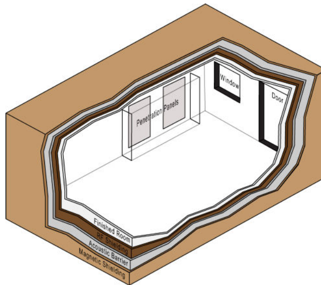
Illustration 2-46: Magnet Room Layers
