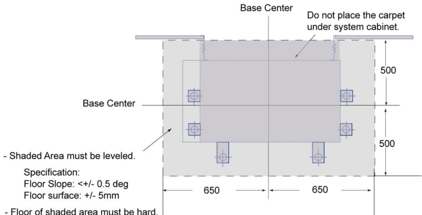
Illustration 2-50: Area to be leveled
