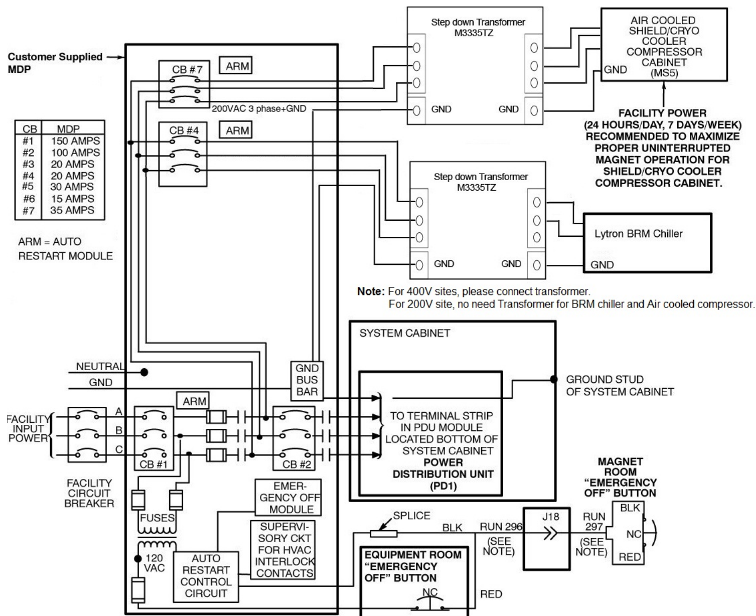
Illustration 5-2: Step down transformer connected method with customer provided MDP (Type D)
