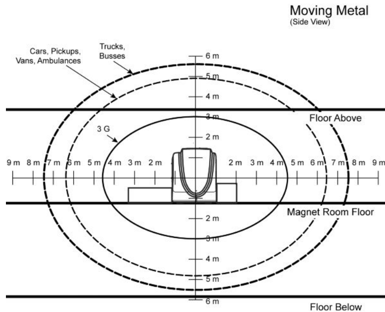
Illustration 3-14: Magnet Moving Metal Sensitivity Line Plot (Side View)
