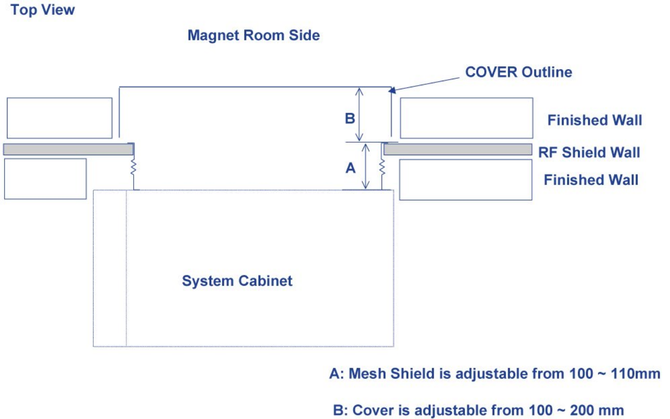
Illustration 3-11: System Cabinet Cover Top View
