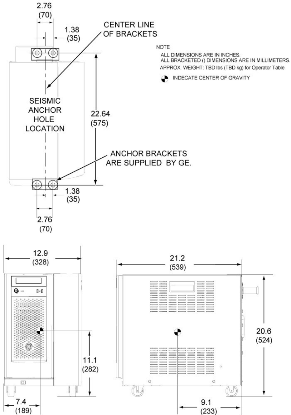
Illustration 2-30: Simple OC Computer Cabinet (OW1 A2)
