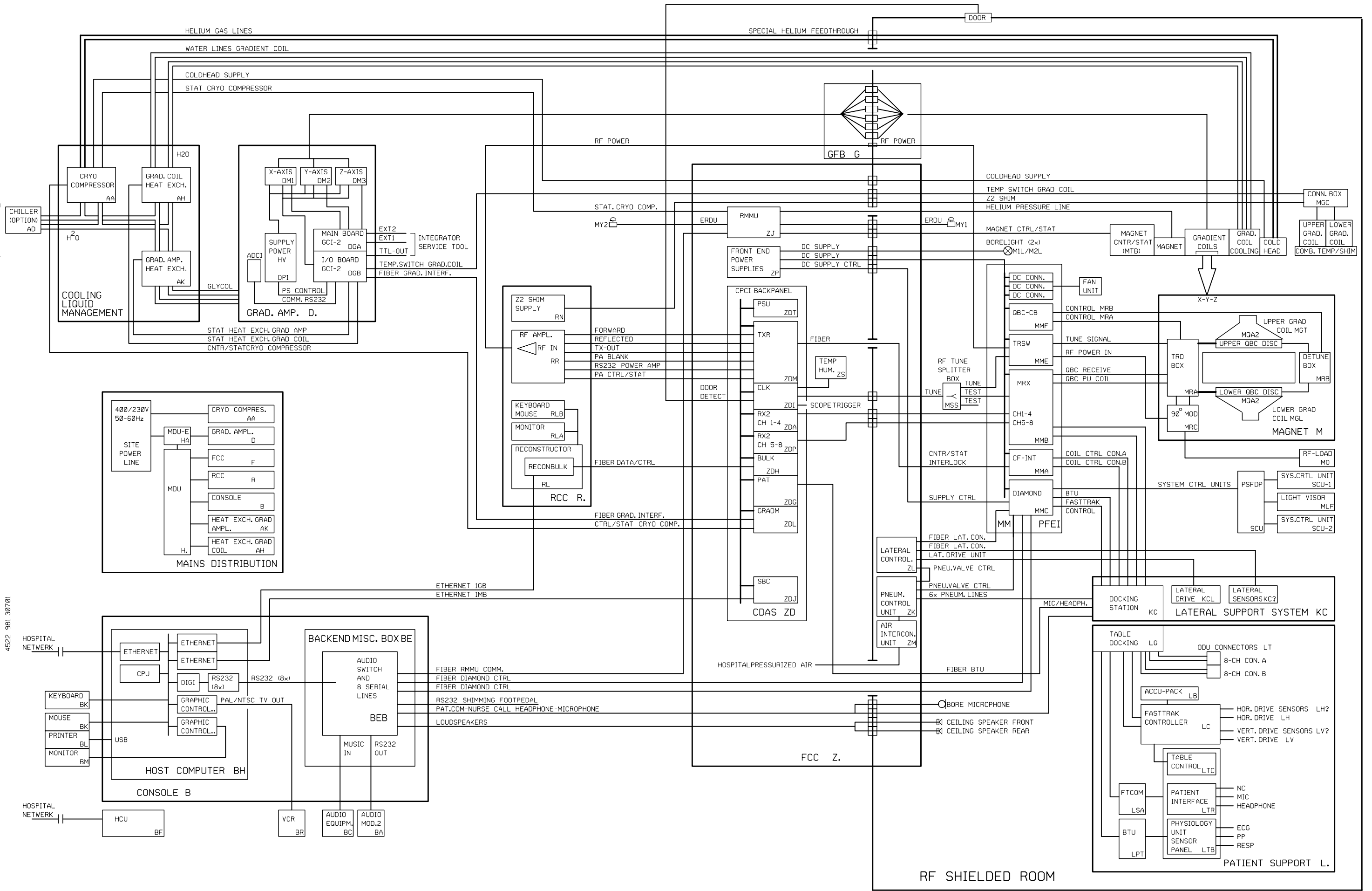
BLOCKDIAGRAM MR SYSTEM
