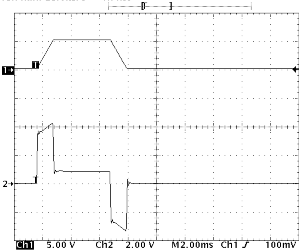
ILLUSTRATION 4-6 AC04 WAVEFORM - UNIPOLAR TRAPEZOID
