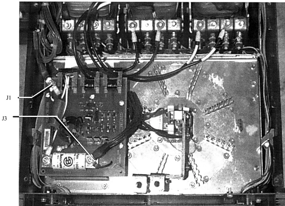
FINAL WIRING ILLUSTRATION 3-13
