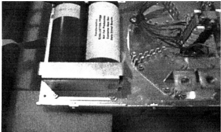
REAR CAPACITOR SUPPORT BRACKET ILLUSTRATION 3-7
