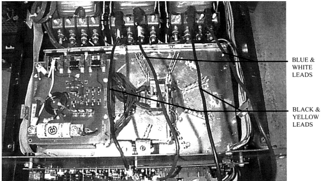
INSTALLING LEAD EXTENSIONS ILLUSTRATION 3-11
