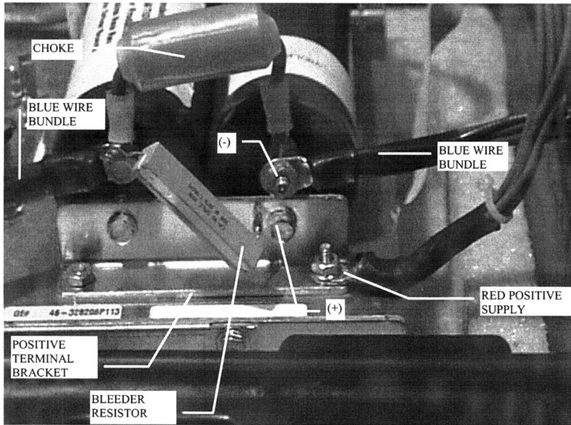
ELECTROLYTIC CAPACITORS ILLUSTRATION 1-5
