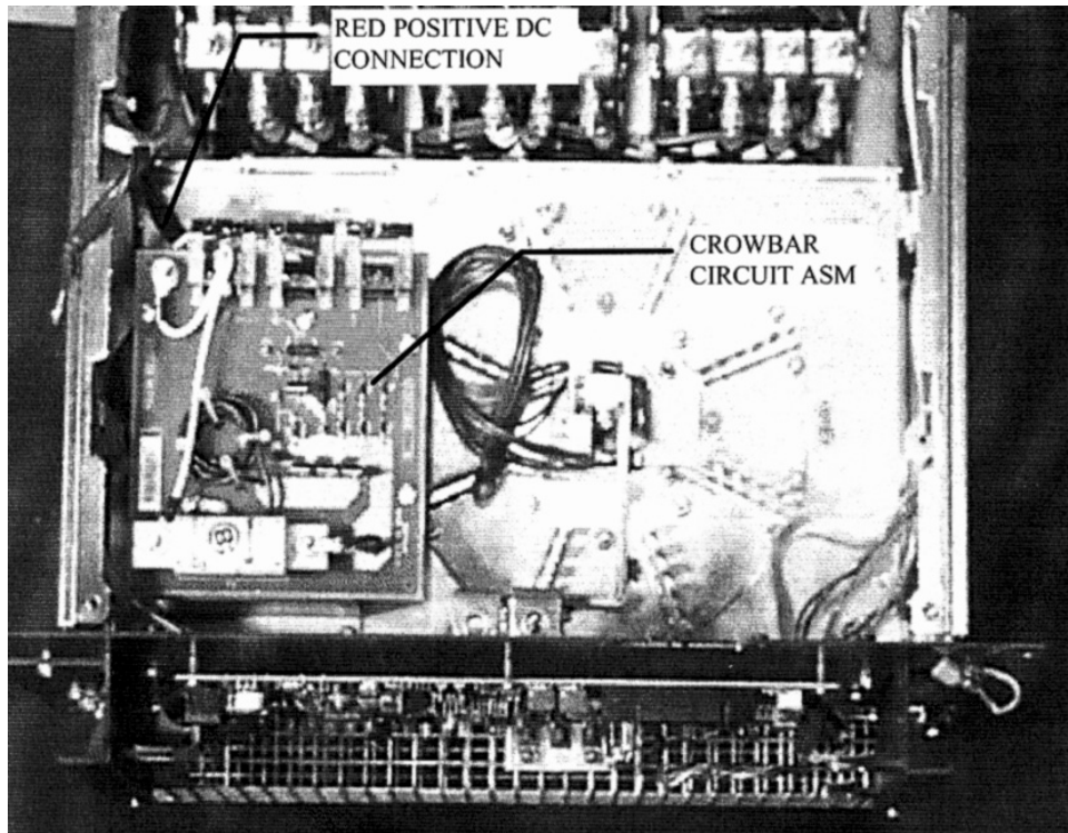
MOUNTING CROWBAR CIRCUIT ILLUSTRATION 3-8
