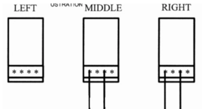
INSTALLING THE CHOKE ILLUSTRATION 3-10
