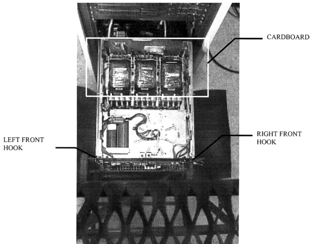
SHELF REMOVED ILLUSTRATION 3-4
