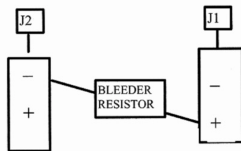
CONNECTING RESISTOR AND LEADS ILLUSTRATION 3-9
