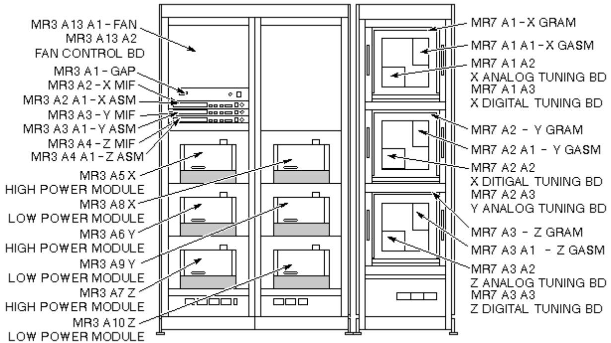
SIGNA HORIZON ECHOSPEED – FRONT VIEW ILLUSTRATION L4749D
