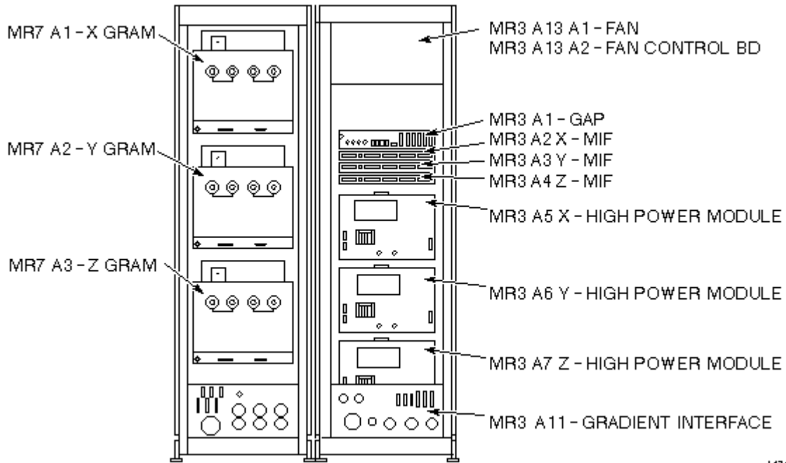
SIGNA HORIZON HISPEED – REAR VIEW ILLUSTRATION L4749B
