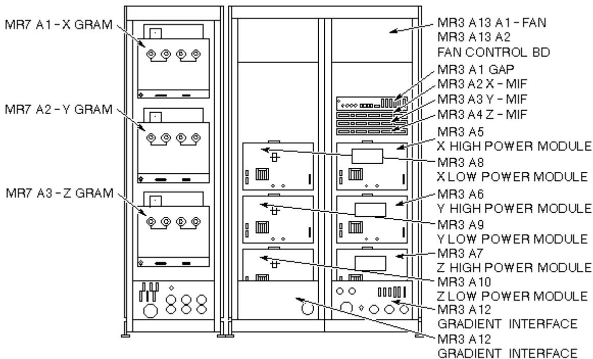
SIGNA HORIZON ECHOSPEED – REAR VIEW ILLUSTRATION L4749A
