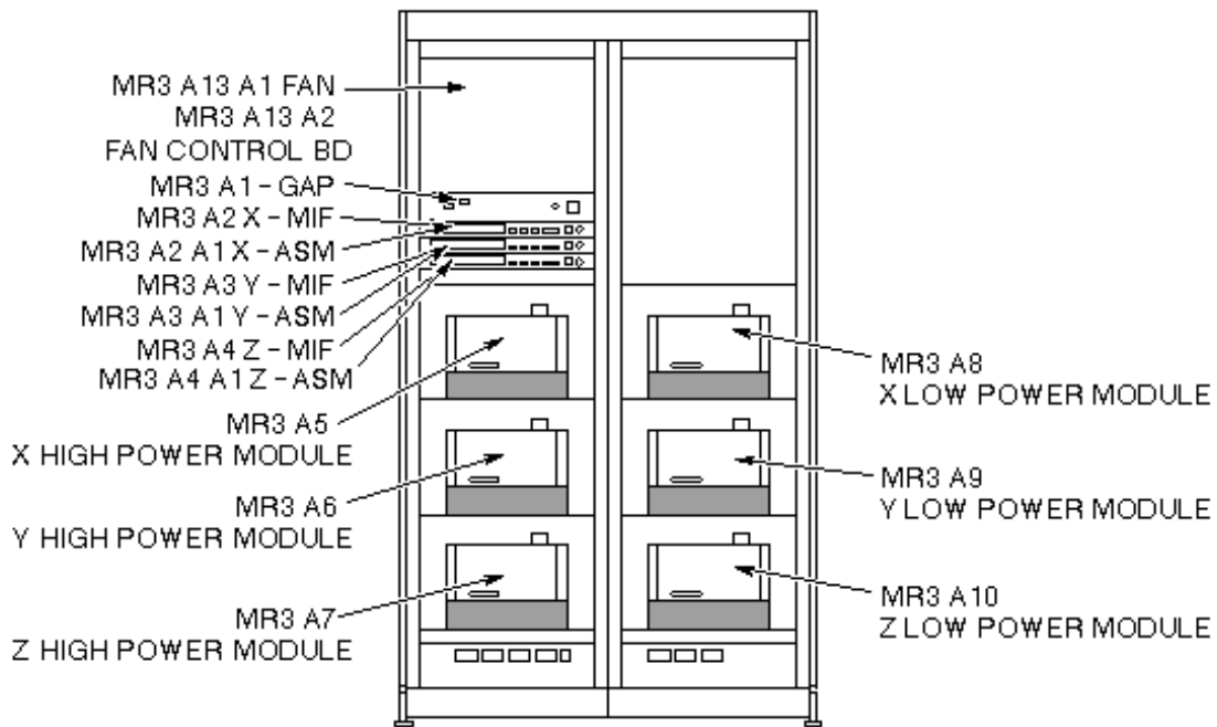
SIGNA HORIZON – FRONT VIEW ILLUSTRATION L4749F
