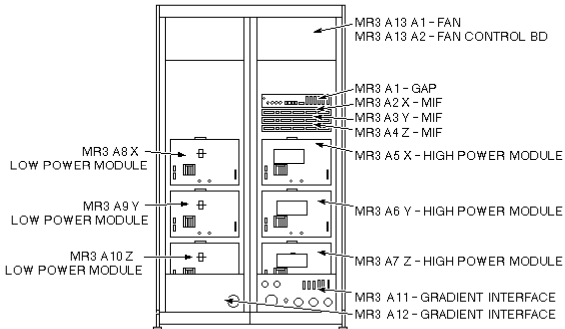
SIGNA HORIZON – REAR VIEW ILLUSTRATION L4749C
