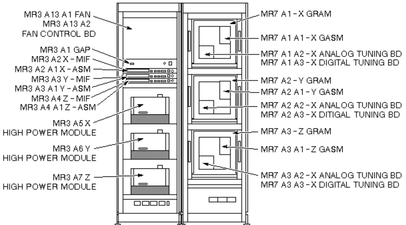
SIGNA HORIZON HISPEED – FRONT VIEW ILLUSTRATION L4749E
