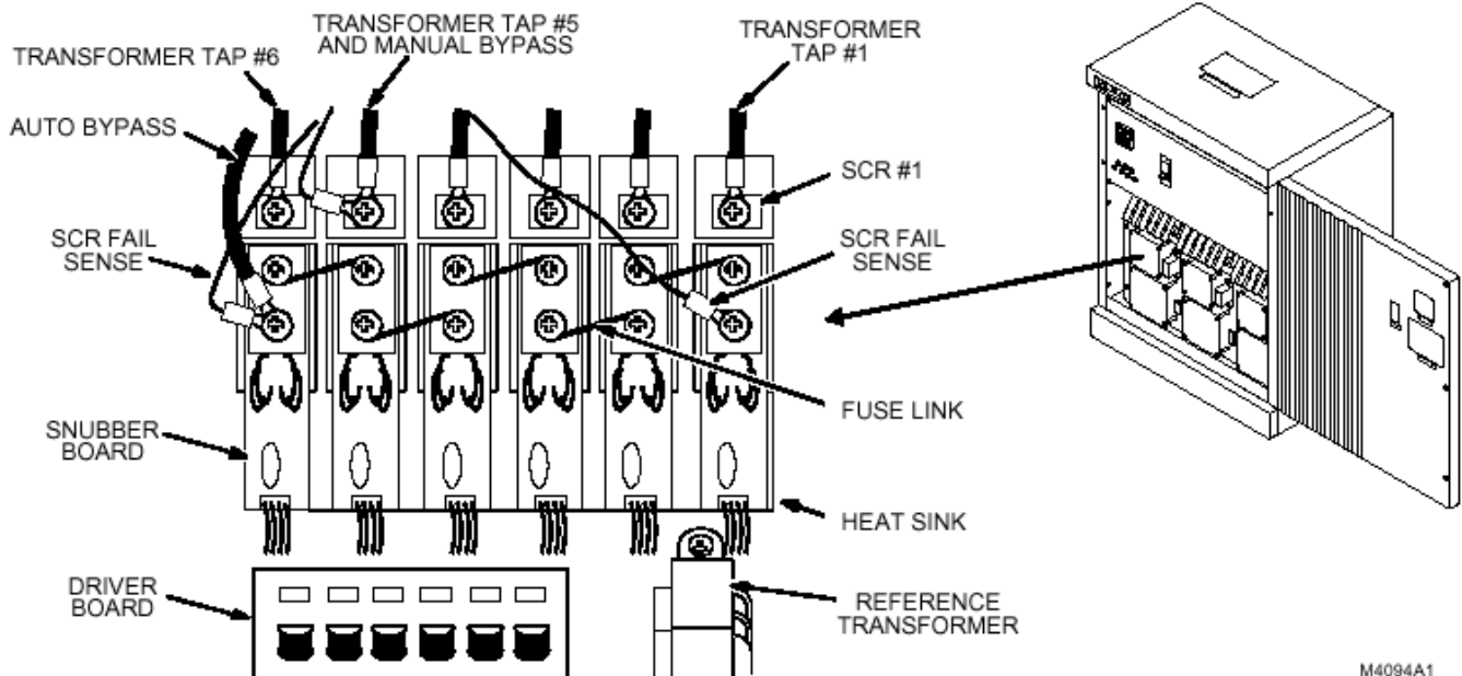
REGULATOR SCR ASSEMBLIES AND SNUBBER BOARDS ILLUSTRATION 5-6
